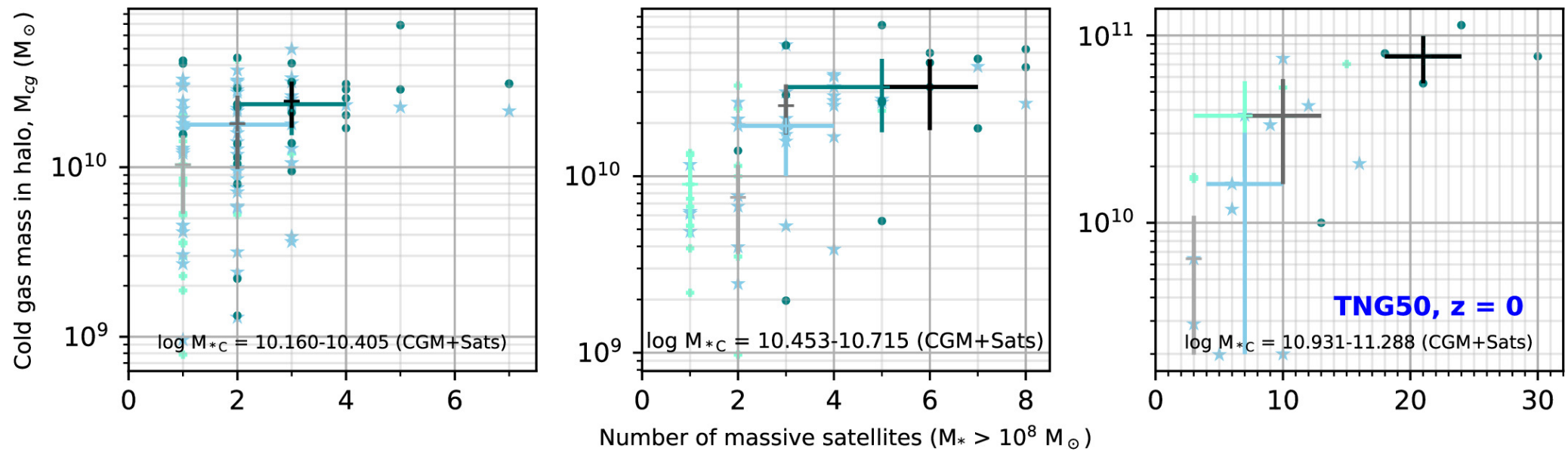
Figure 5. from Mitali Damle et al 2025 Astrophys. J. 986 doi:10.3847/1538-4357/adcee9 https://dx.doi.org/10.3847/1538-4357/adcee9 © 2025. The Author(s). Published by the American Astronomical Society.
