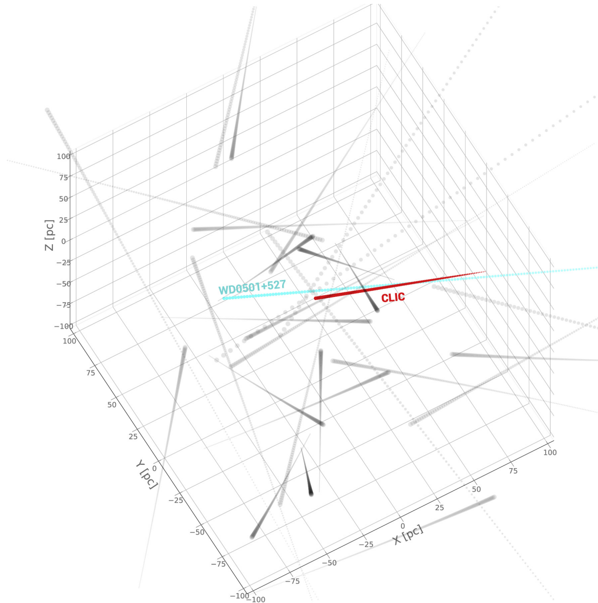
Figure 9. from Catherine Zucker et al 2025 Astrophys. J. 986 doi:10.3847/1538-4357/adc920 https://dx.doi.org/10.3847/1538-4357/adc920 © 2025. The Author(s). Published by the American Astronomical Society.
