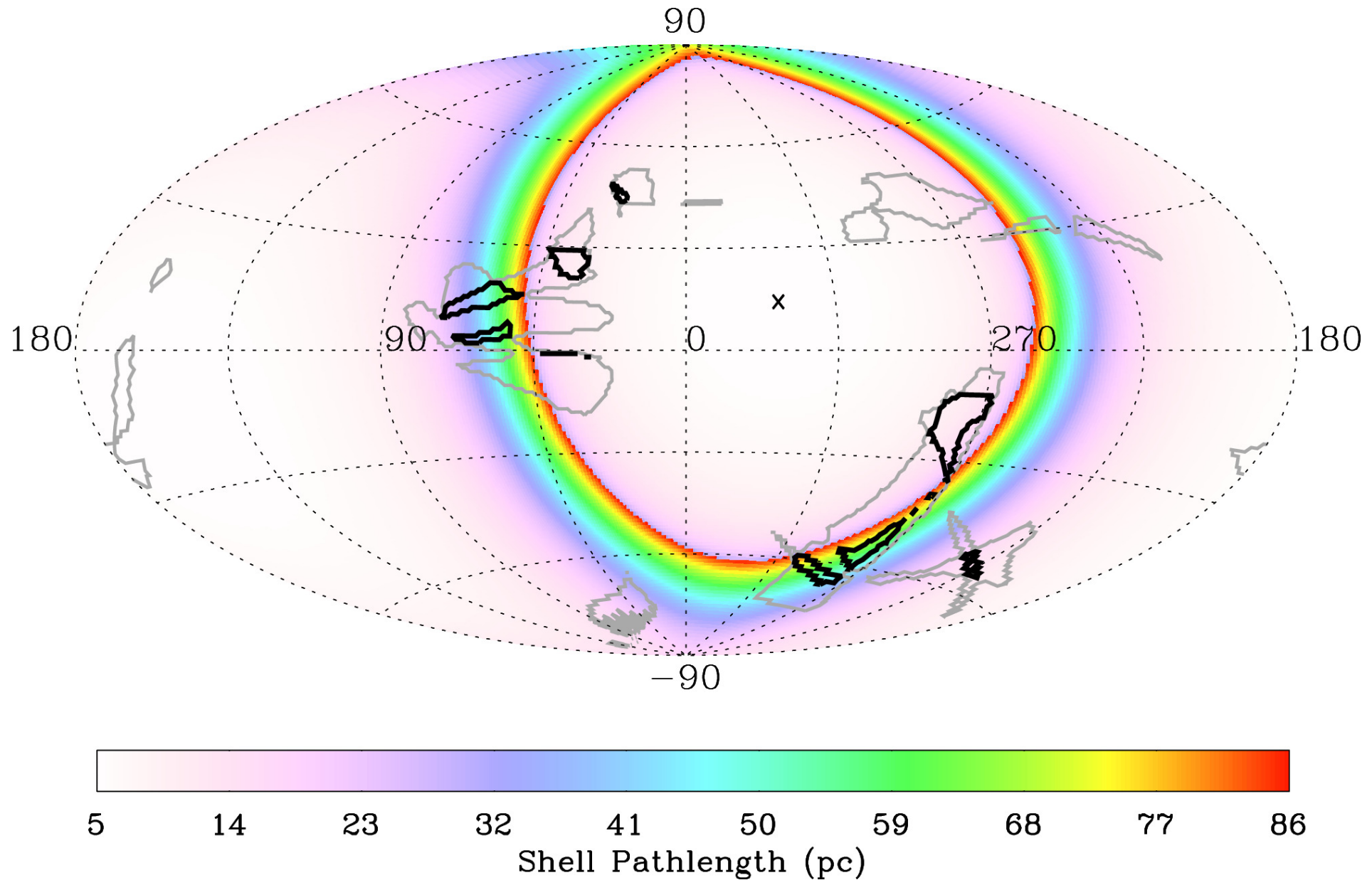
Figure 8. from Catherine Zucker et al 2025 Astrophys. J. 986 doi:10.3847/1538-4357/adc920 https://dx.doi.org/10.3847/1538-4357/adc920 © 2025. The Author(s). Published by the American Astronomical Society.
