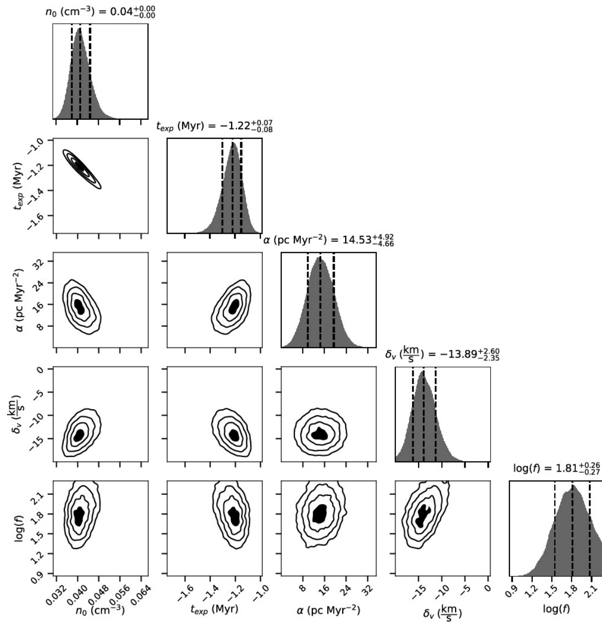
Figure 4. from Catherine Zucker et al 2025 Astrophys. J. 986 doi:10.3847/1538-4357/adc920 https://dx.doi.org/10.3847/1538-4357/adc920 © 2025. The Author(s). Published by the American Astronomical Society.
