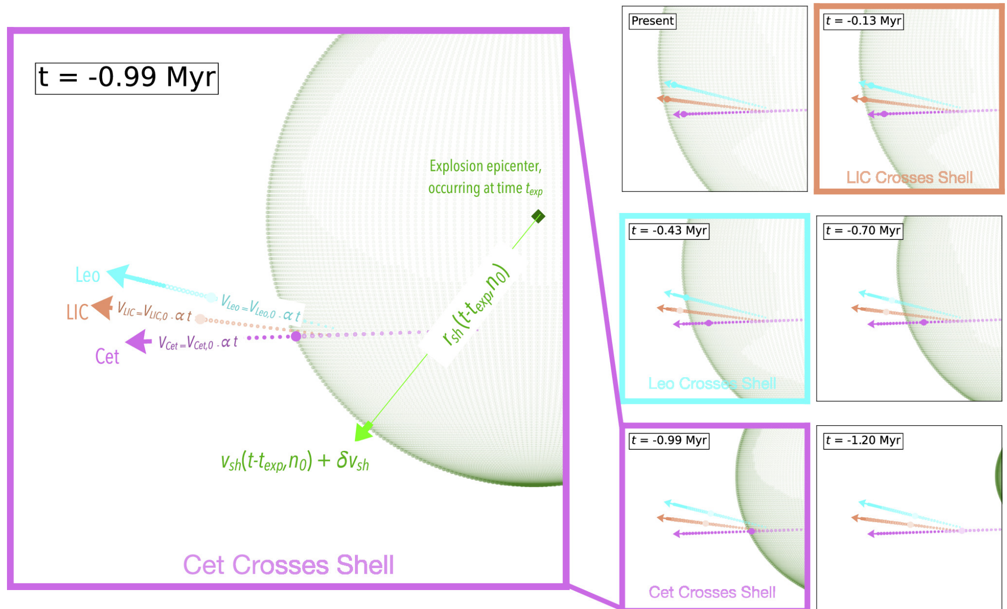
Figure 3. from Catherine Zucker et al 2025 Astrophys. J. 986 doi:10.3847/1538-4357/adc920 https://dx.doi.org/10.3847/1538-4357/adc920 © 2025. The Author(s). Published by the American Astronomical Society.
