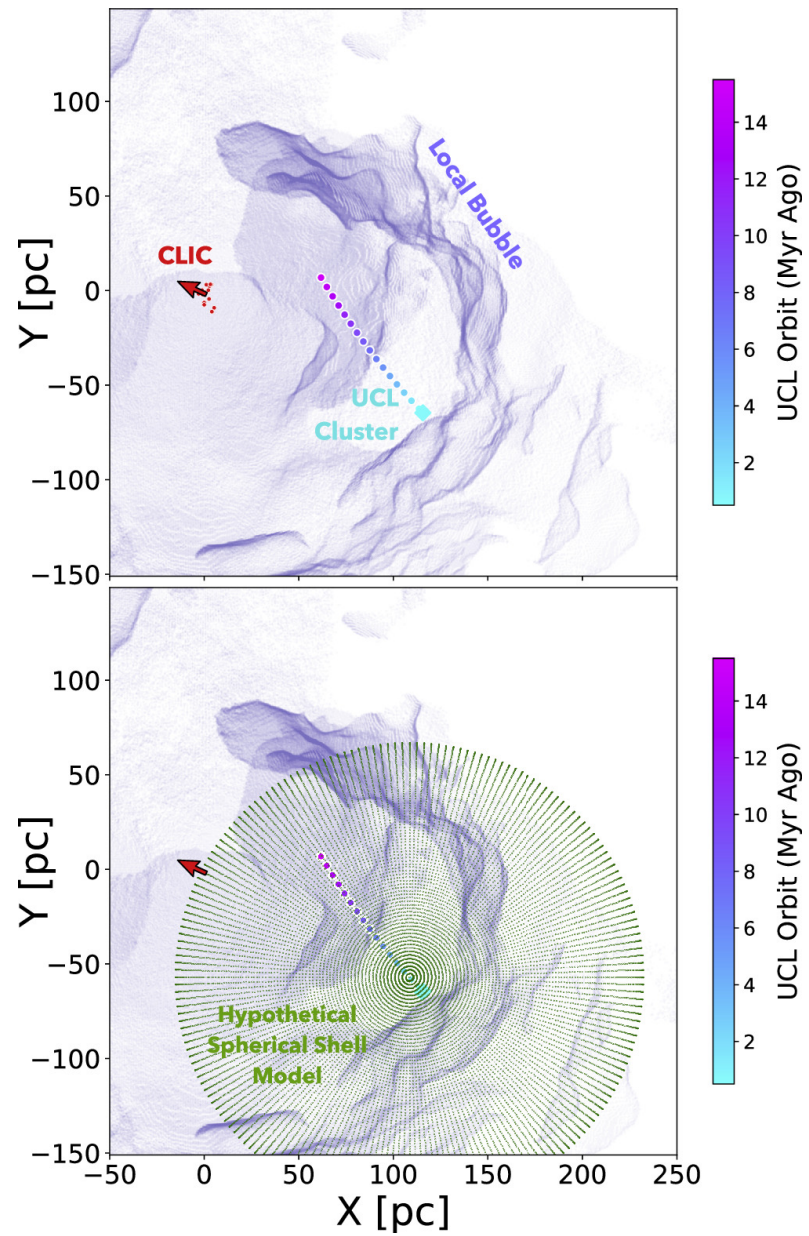
Figure 2. from Catherine Zucker et al 2025 Astrophys. J. 986 doi:10.3847/1538-4357/adc920 https://dx.doi.org/10.3847/1538-4357/adc920 © 2025. The Author(s). Published by the American Astronomical Society.
