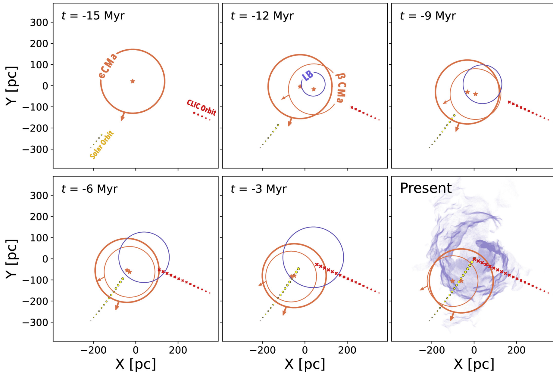
Figure 10. from Catherine Zucker et al 2025 Astrophys. J. 986 doi:10.3847/1538-4357/adc920 https://dx.doi.org/10.3847/1538-4357/adc920 © 2025. The Author(s). Published by the American Astronomical Society.
