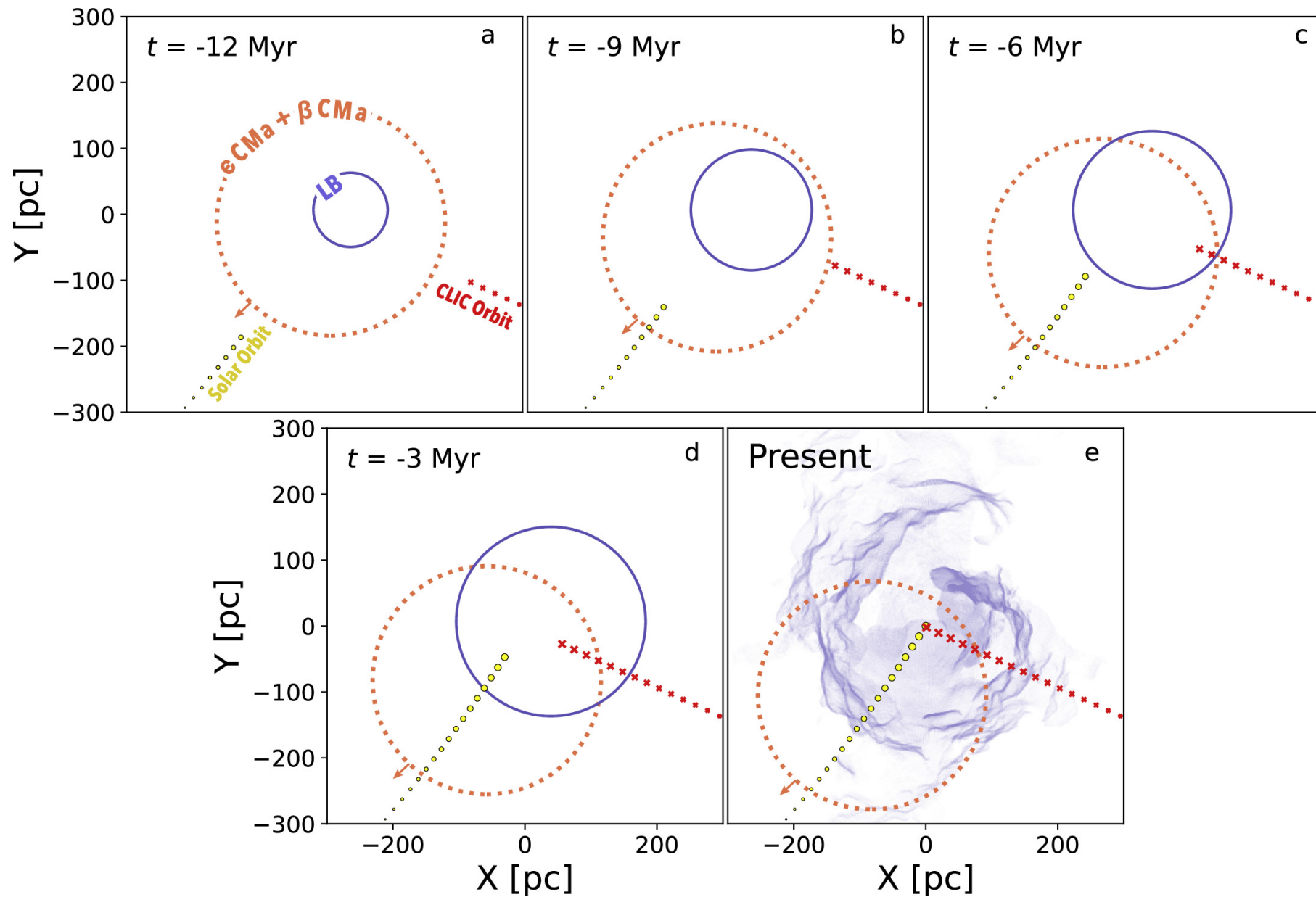
Figure 1. from Catherine Zucker et al 2025 Astrophys. J. 986 doi:10.3847/1538-4357/adc920 https://dx.doi.org/10.3847/1538-4357/adc920 © 2025. The Author(s). Published by the American Astronomical Society.
