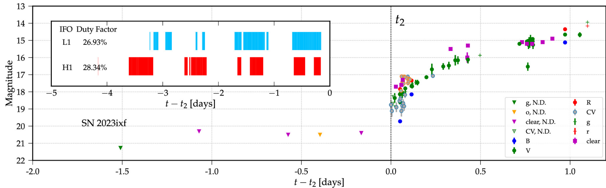
Figure 1. from A. G. Abac et al 2025 Astrophys. J. 985 doi:10.3847/1538-4357/adc681 https://dx.doi.org/10.3847/1538-4357/adc681 © 2025. The Author(s). Published by the American Astronomical Society.
