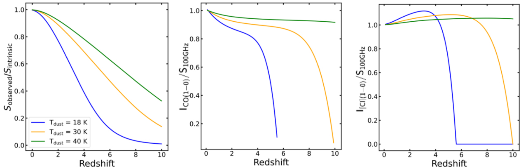
Figure 9. from Marta Frias Castillo et al 2025 Astrophys. J. 987 doi:10.3847/1538-4357/adc4e0 https://dx.doi.org/10.3847/1538-4357/adc4e0 © 2025. The Author(s). Published by the American Astronomical Society.
