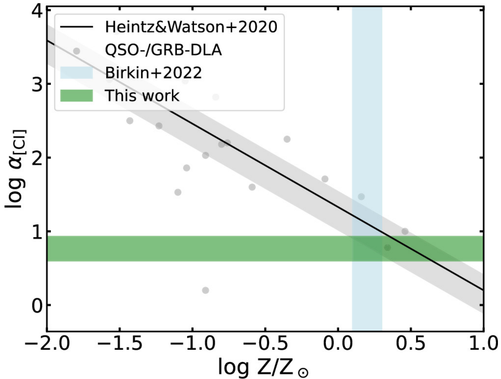
Figure 8. from Marta Frias Castillo et al 2025 Astrophys. J. 987 doi:10.3847/1538-4357/adc4e0 https://dx.doi.org/10.3847/1538-4357/adc4e0 © 2025. The Author(s). Published by the American Astronomical Society.
