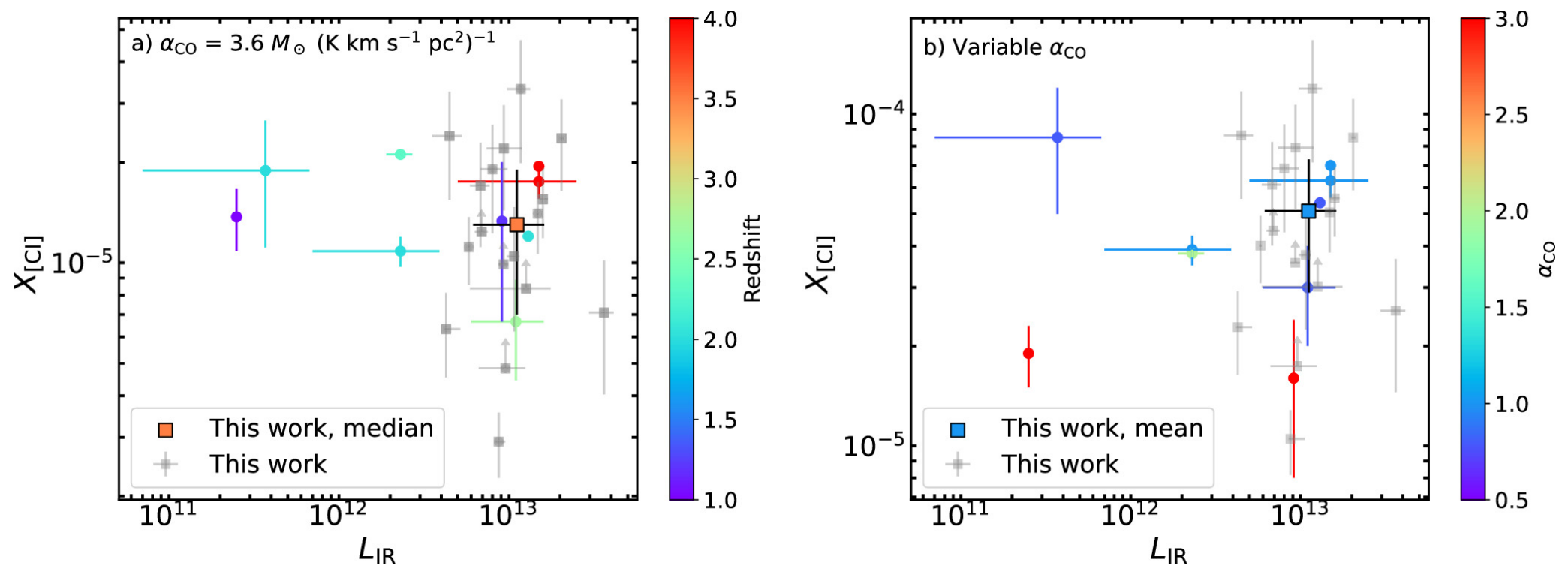
Figure 7. from Marta Frias Castillo et al 2025 Astrophys. J. 987 doi:10.3847/1538-4357/adc4e0 https://dx.doi.org/10.3847/1538-4357/adc4e0 © 2025. The Author(s). Published by the American Astronomical Society.
