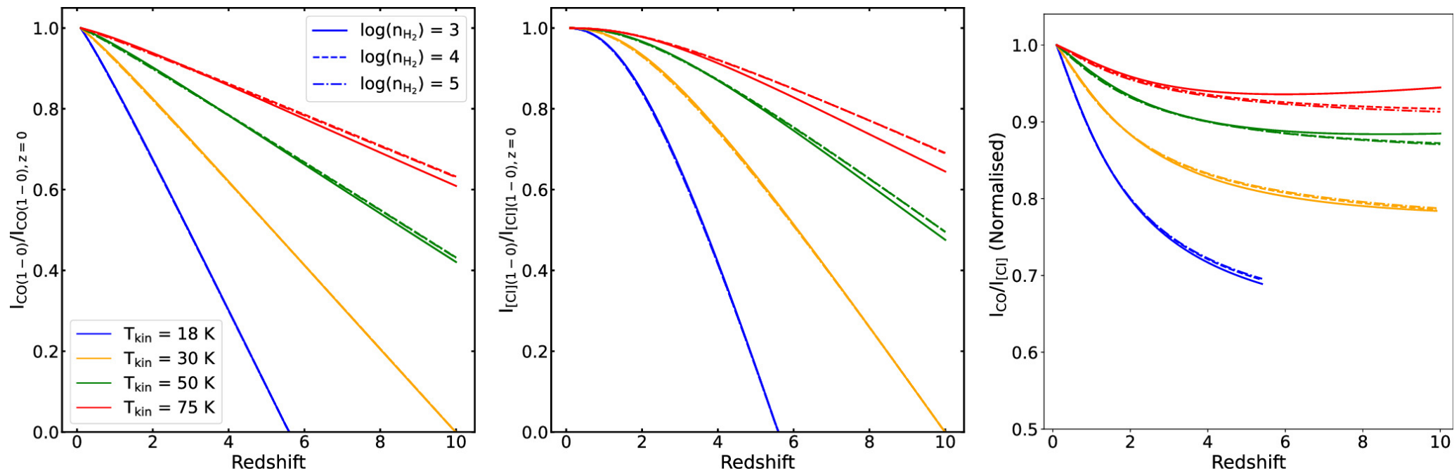
Figure 6. from Marta Frias Castillo et al 2025 Astrophys. J. 987 doi:10.3847/1538-4357/adc4e0 https://dx.doi.org/10.3847/1538-4357/adc4e0 © 2025. The Author(s). Published by the American Astronomical Society.
