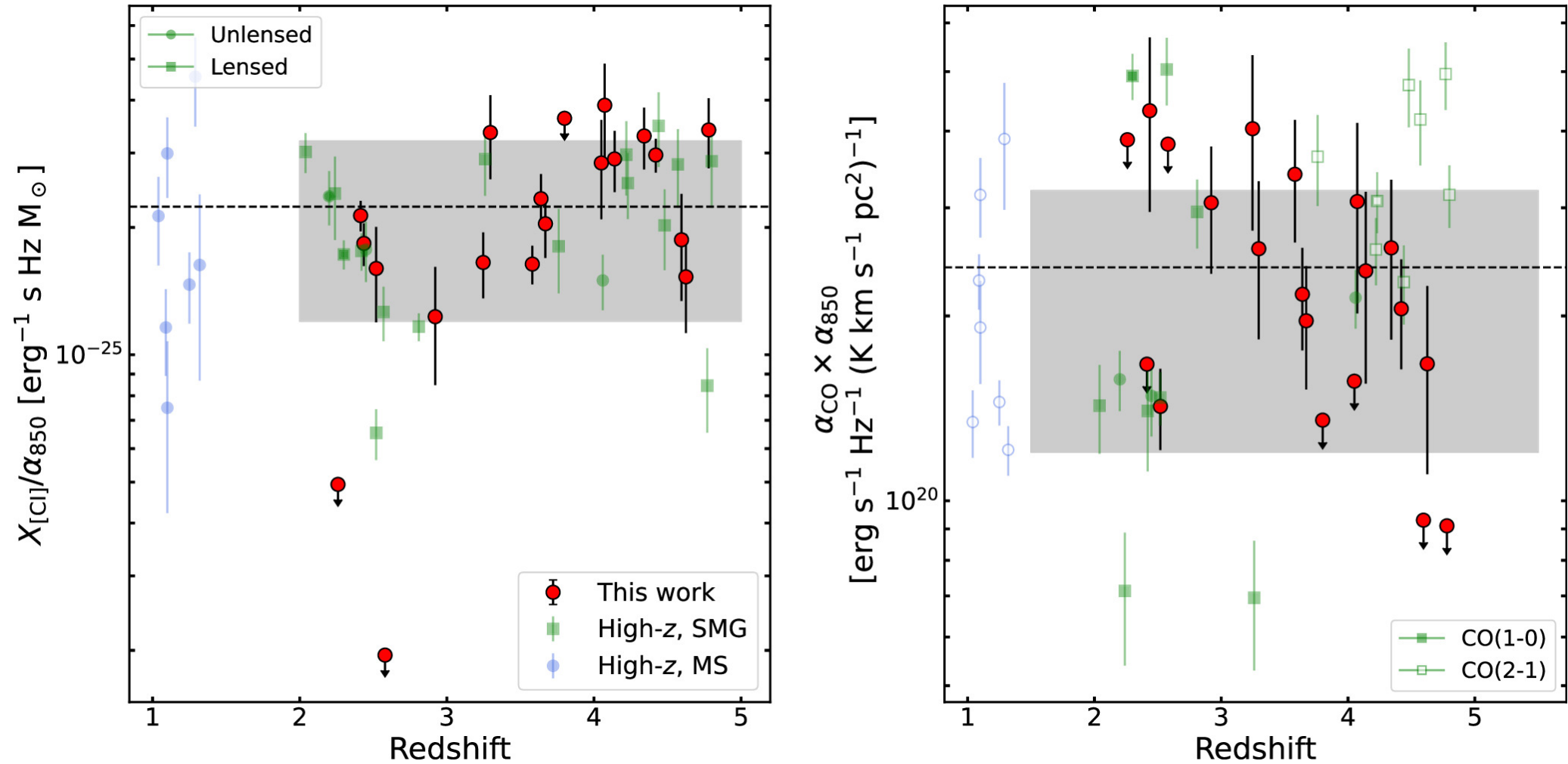
Figure 5. from Marta Frias Castillo et al 2025 Astrophys. J. 987 doi:10.3847/1538-4357/adc4e0 https://dx.doi.org/10.3847/1538-4357/adc4e0 © 2025. The Author(s). Published by the American Astronomical Society.
