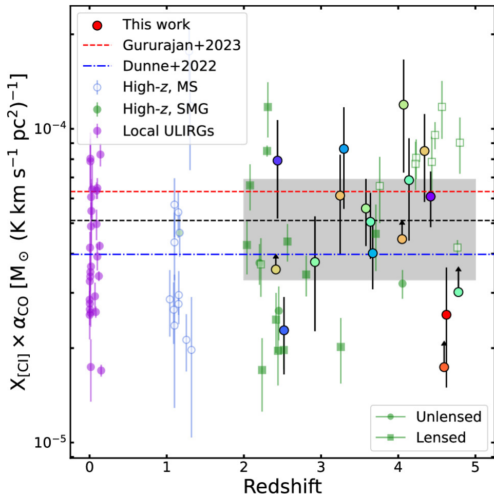
Figure 4. from Marta Frias Castillo et al 2025 Astrophys. J. 987 doi:10.3847/1538-4357/adc4e0 https://dx.doi.org/10.3847/1538-4357/adc4e0 © 2025. The Author(s). Published by the American Astronomical Society.
