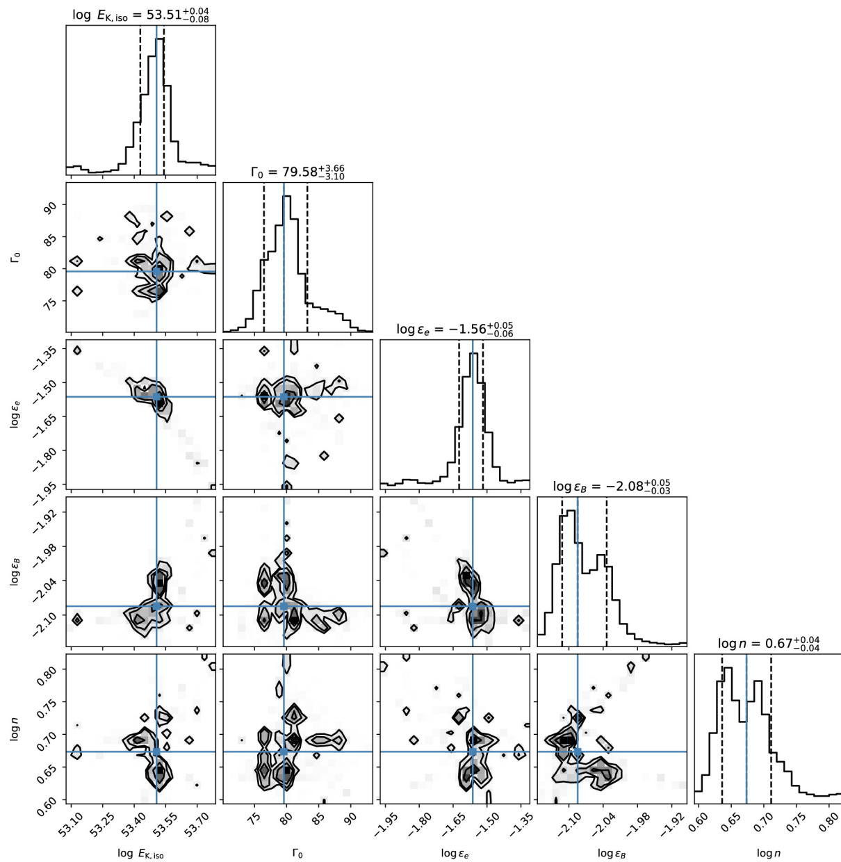
Figure 9. from Zi-Min Zhou et al 2025 Astrophys. J. 984 doi:10.3847/1538-4357/adc45c https://dx.doi.org/10.3847/1538-4357/adc45c © 2025. The Author(s). Published by the American Astronomical Society.
