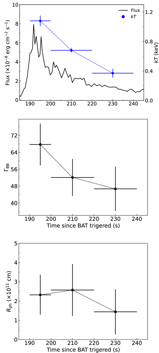
Figure 7. from Zi-Min Zhou et al 2025 Astrophys. J. 984 doi:10.3847/1538-4357/adc45c https://dx.doi.org/10.3847/1538-4357/adc45c © 2025. The Author(s). Published by the American Astronomical Society.
