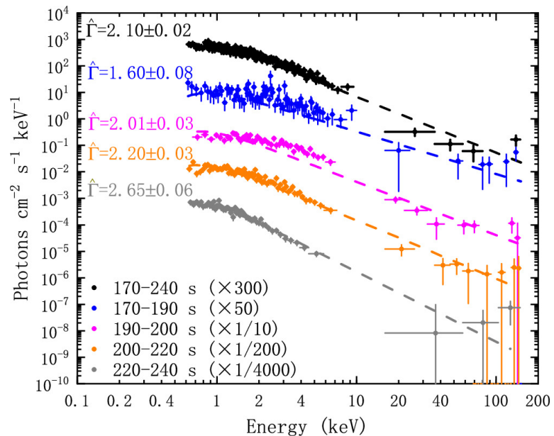
Figure 5. from Zi-Min Zhou et al 2025 Astrophys. J. 984 doi:10.3847/1538-4357/adc45c https://dx.doi.org/10.3847/1538-4357/adc45c © 2025. The Author(s). Published by the American Astronomical Society.
