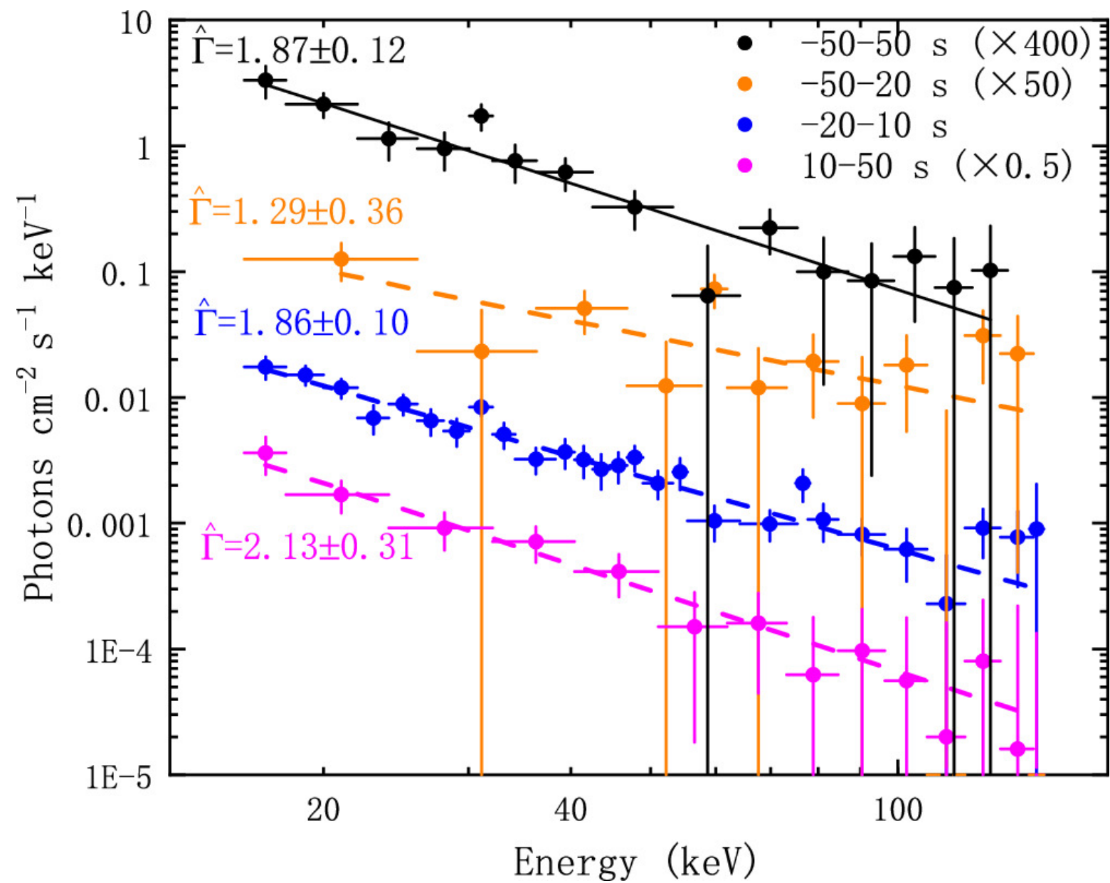
Figure 3. from Zi-Min Zhou et al 2025 Astrophys. J. 984 doi:10.3847/1538-4357/adc45c https://dx.doi.org/10.3847/1538-4357/adc45c © 2025. The Author(s). Published by the American Astronomical Society.
