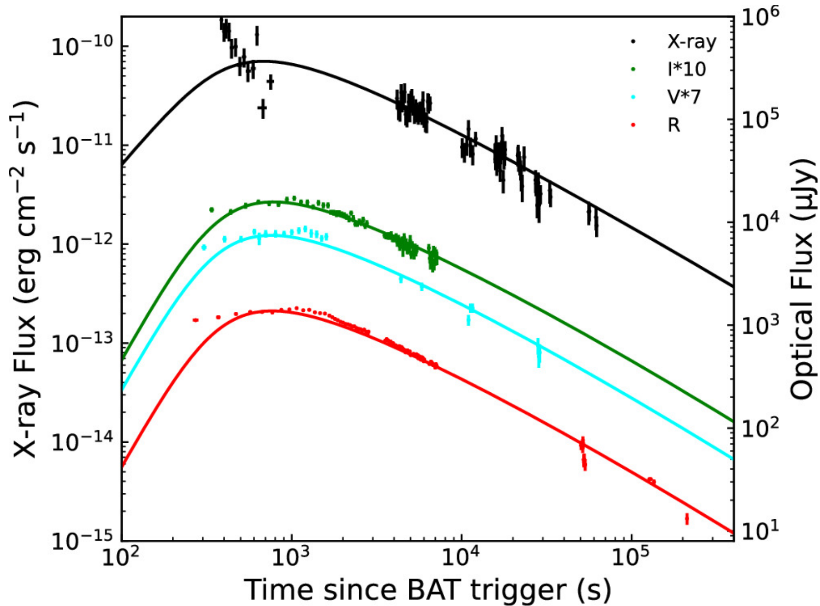
Figure 10. from Zi-Min Zhou et al 2025 Astrophys. J. 984 doi:10.3847/1538-4357/adc45c https://dx.doi.org/10.3847/1538-4357/adc45c © 2025. The Author(s). Published by the American Astronomical Society.
