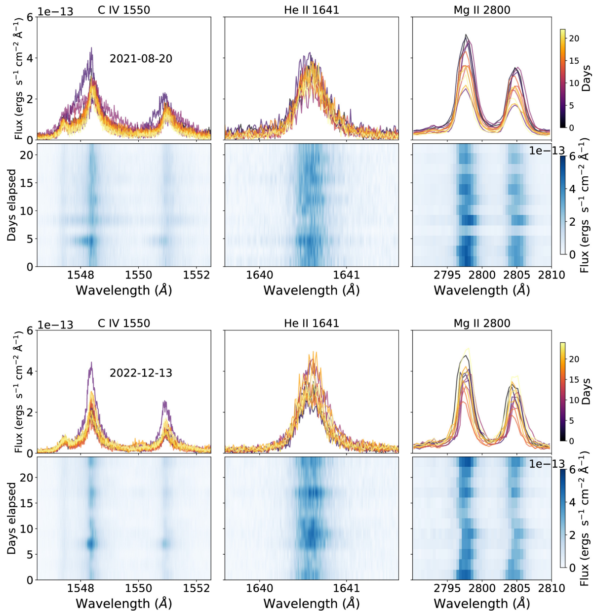
Figure 5. from Julia Roman-Duval et al 2025 Astrophys. J. 985 doi:10.3847/1538-4357/adc45b https://dx.doi.org/10.3847/1538-4357/adc45b © 2025. The Author(s). Published by the American Astronomical Society.
