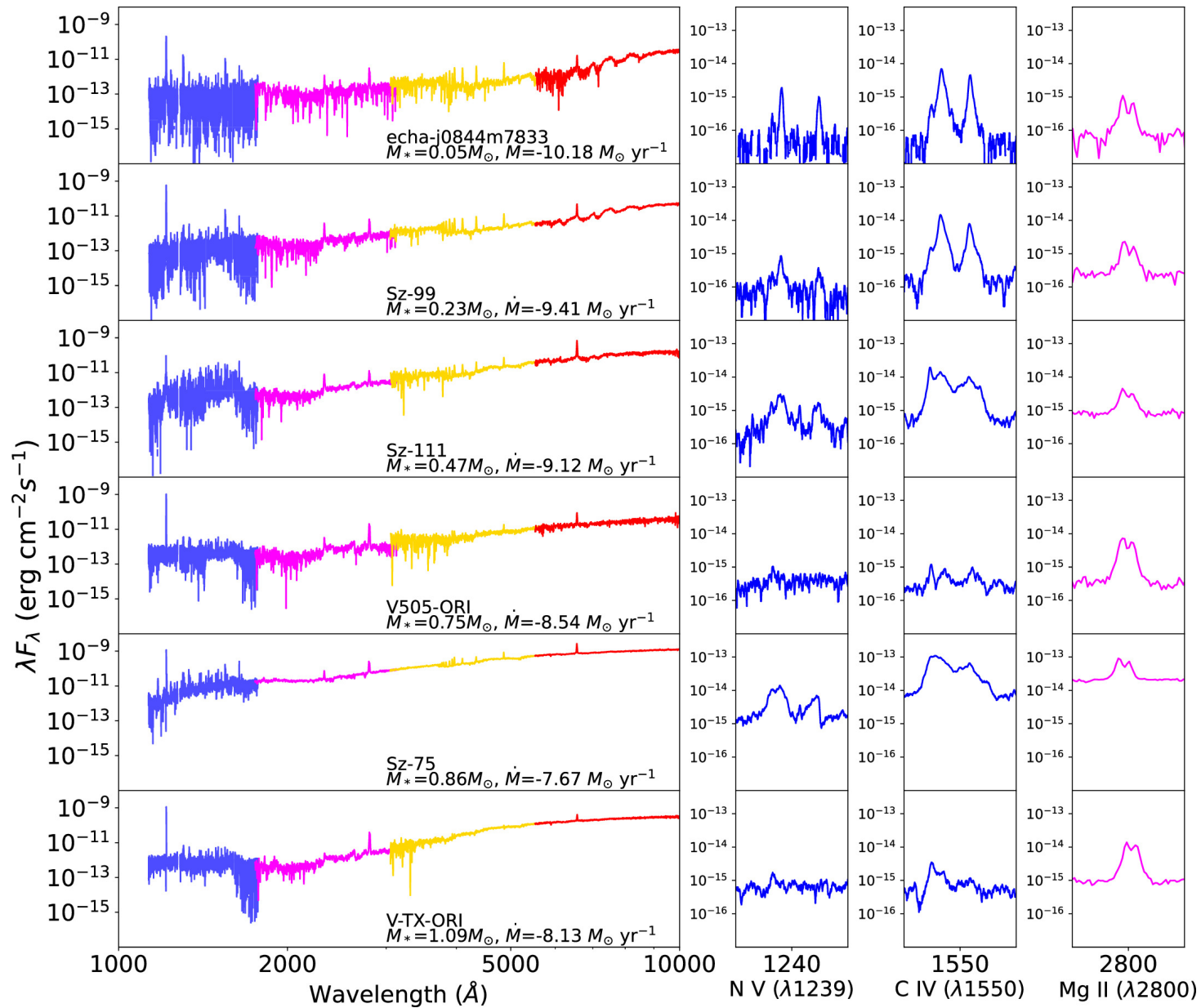
Figure 4. from Julia Roman-Duval et al 2025 Astrophys. J. 985 doi:10.3847/1538-4357/adc45b https://dx.doi.org/10.3847/1538-4357/adc45b © 2025. The Author(s). Published by the American Astronomical Society.
