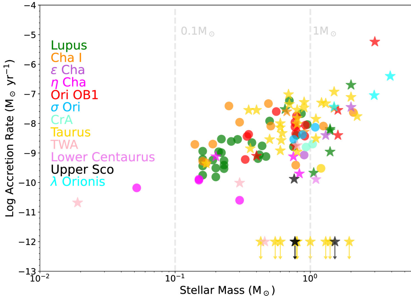
Figure 3. from Julia Roman-Duval et al 2025 Astrophys. J. 985 doi:10.3847/1538-4357/adc45b https://dx.doi.org/10.3847/1538-4357/adc45b © 2025. The Author(s). Published by the American Astronomical Society.
