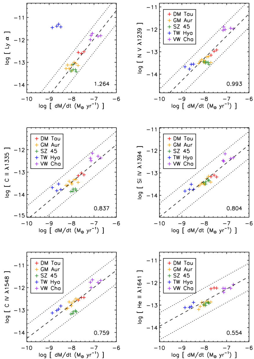
Figure 17. from Julia Roman-Duval et al 2025 Astrophys. J. 985 doi:10.3847/1538-4357/adc45b https://dx.doi.org/10.3847/1538-4357/adc45b © 2025. The Author(s). Published by the American Astronomical Society.
