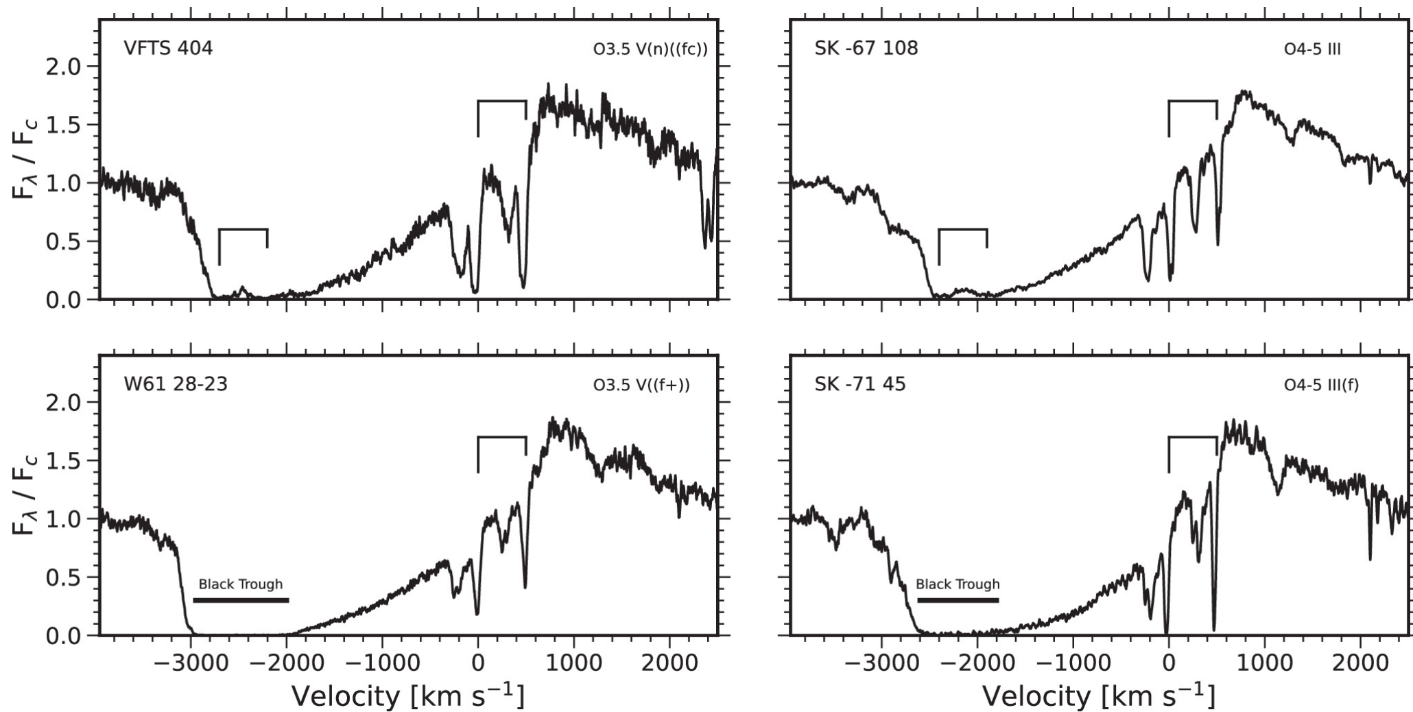
Figure 14. from Julia Roman-Duval et al 2025 Astrophys. J. 985 doi:10.3847/1538-4357/adc45b https://dx.doi.org/10.3847/1538-4357/adc45b © 2025. The Author(s). Published by the American Astronomical Society.
