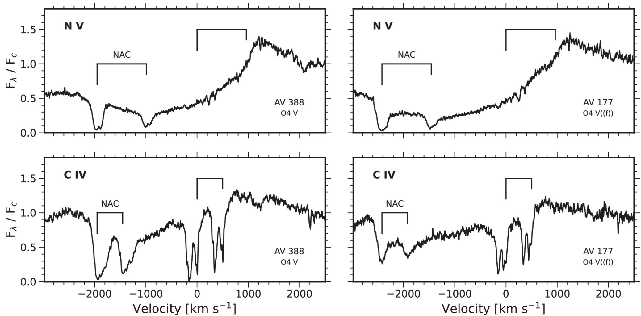
Figure 13. from Julia Roman-Duval et al 2025 Astrophys. J. 985 doi:10.3847/1538-4357/adc45b https://dx.doi.org/10.3847/1538-4357/adc45b © 2025. The Author(s). Published by the American Astronomical Society.
