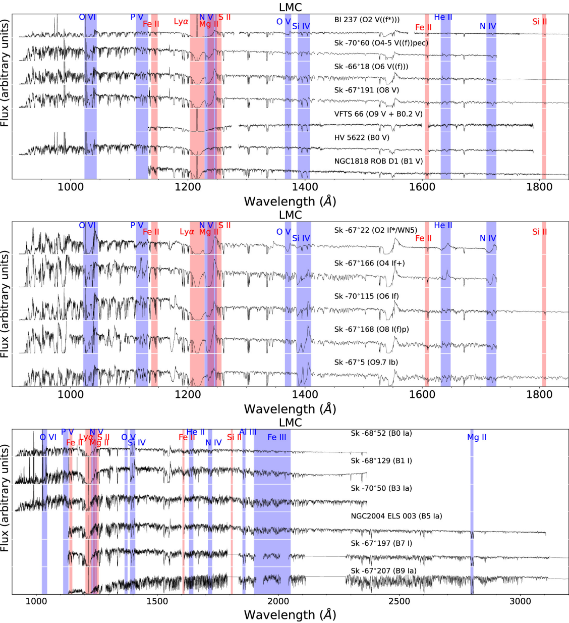
Figure 10. from Julia Roman-Duval et al 2025 Astrophys. J. 985 doi:10.3847/1538-4357/adc45b https://dx.doi.org/10.3847/1538-4357/adc45b © 2025. The Author(s). Published by the American Astronomical Society.
