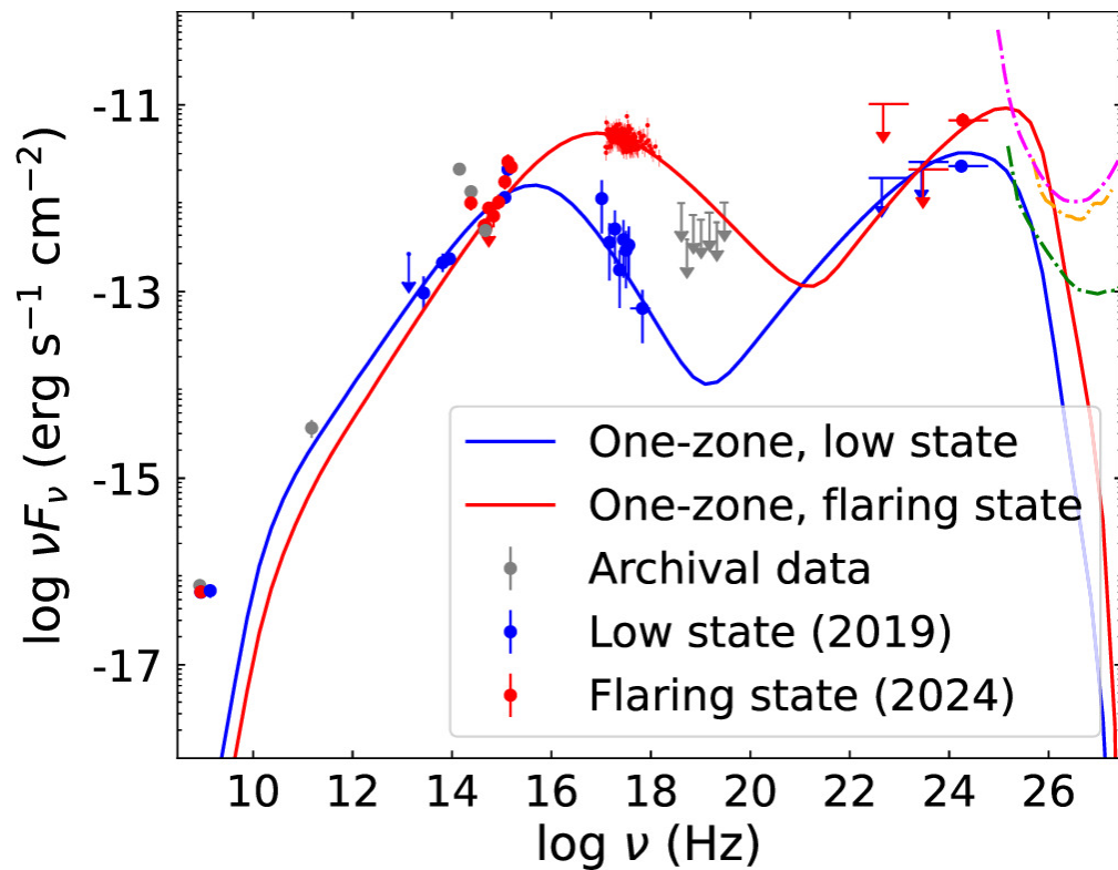
Figure 3. from Mingjun Liu et al 2025 Astrophys. J. 984 doi:10.3847/1538-4357/adc301 https://dx.doi.org/10.3847/1538-4357/adc301 © 2025. The Author(s). Published by the American Astronomical Society.
