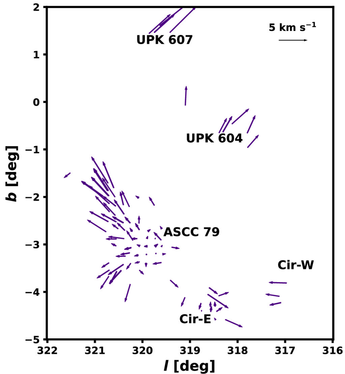
Figure 9. from Ronan Kerr et al 2025 Astrophys. J. 985 doi:10.3847/1538-4357/adc0a7 https://dx.doi.org/10.3847/1538-4357/adc0a7 © 2025. The Author(s). Published by the American Astronomical Society.
