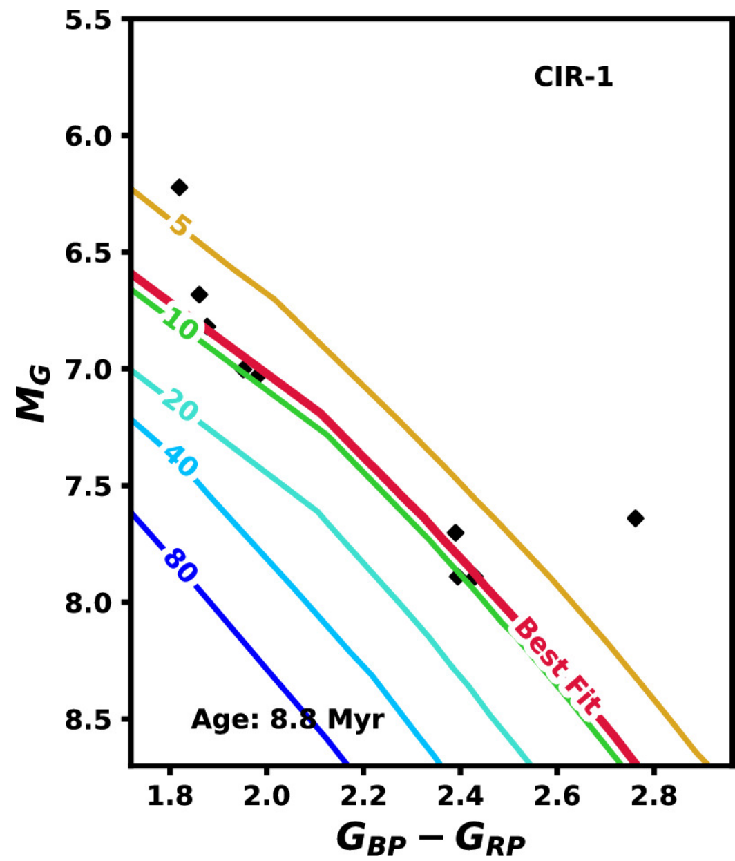
Figure 6. Color–magnitude diagram and Age fit from Ronan Kerr et al 2025 Astrophys. J. 985 doi:10.3847/1538-4357/adc0a7 https://dx.doi.org/10.3847/1538-4357/adc0a7 © 2025. The Author(s). Published by the American Astronomical Society.
