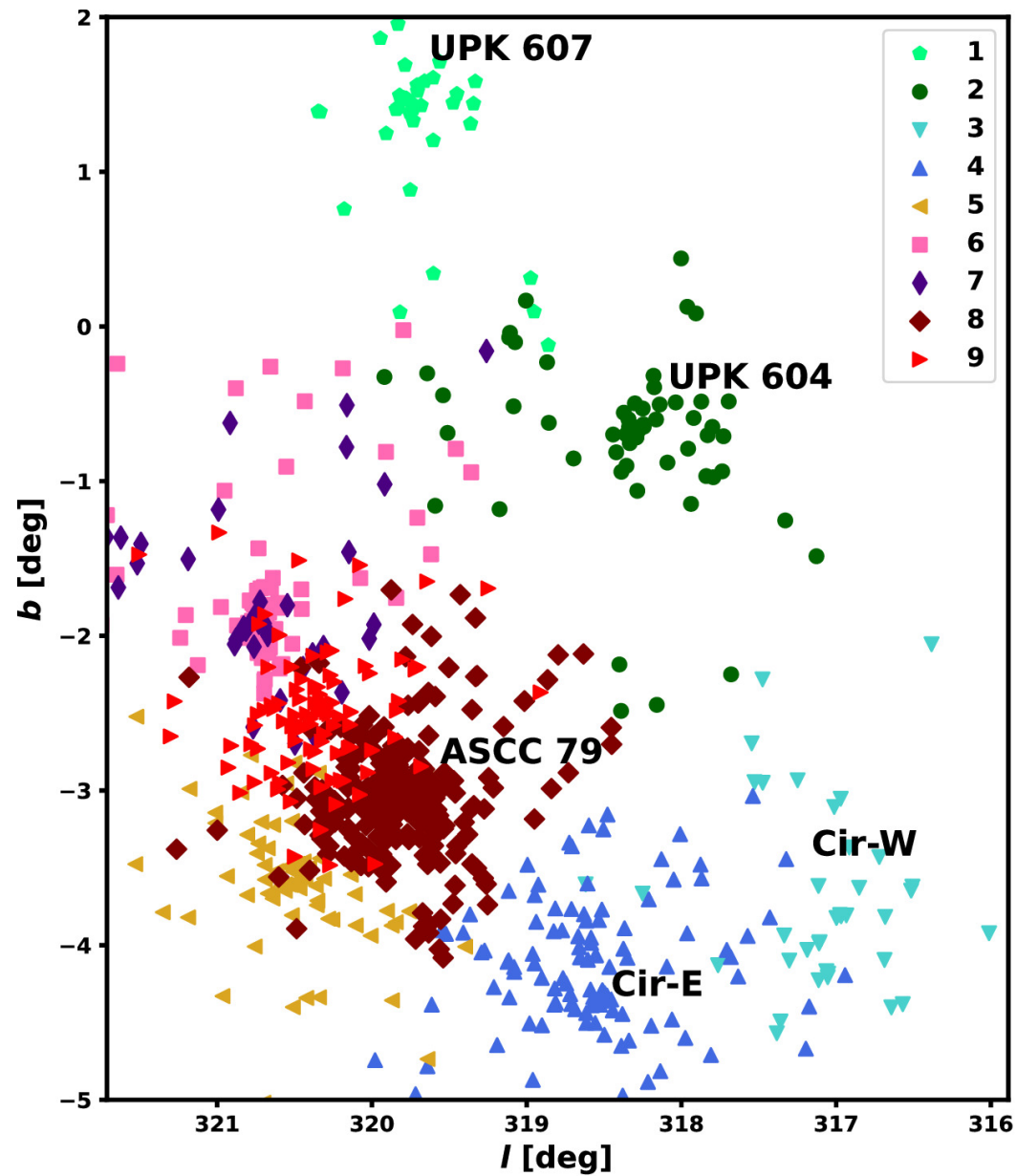
Figure 5. from Ronan Kerr et al 2025 Astrophys. J. 985 doi:10.3847/1538-4357/adc0a7 https://dx.doi.org/10.3847/1538-4357/adc0a7 © 2025. The Author(s). Published by the American Astronomical Society.
