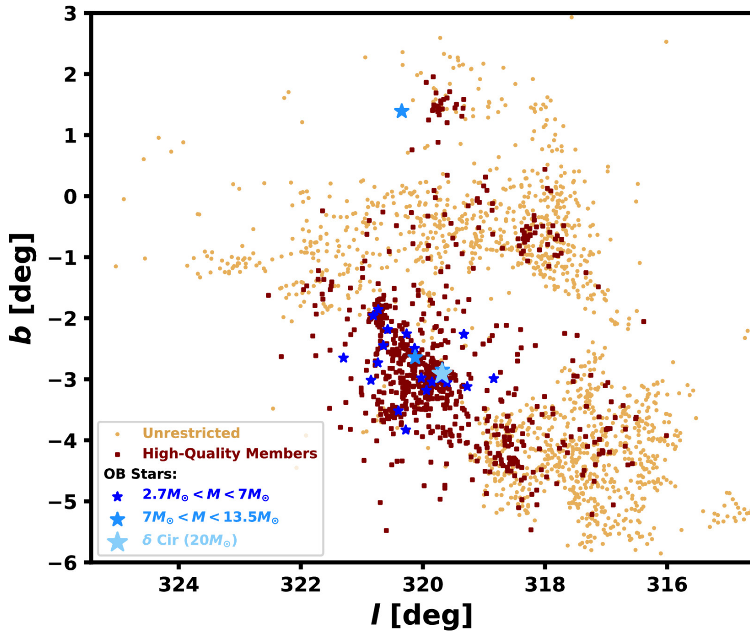
Figure 3. from Ronan Kerr et al 2025 Astrophys. J. 985 doi:10.3847/1538-4357/adc0a7 https://dx.doi.org/10.3847/1538-4357/adc0a7 © 2025. The Author(s). Published by the American Astronomical Society.
