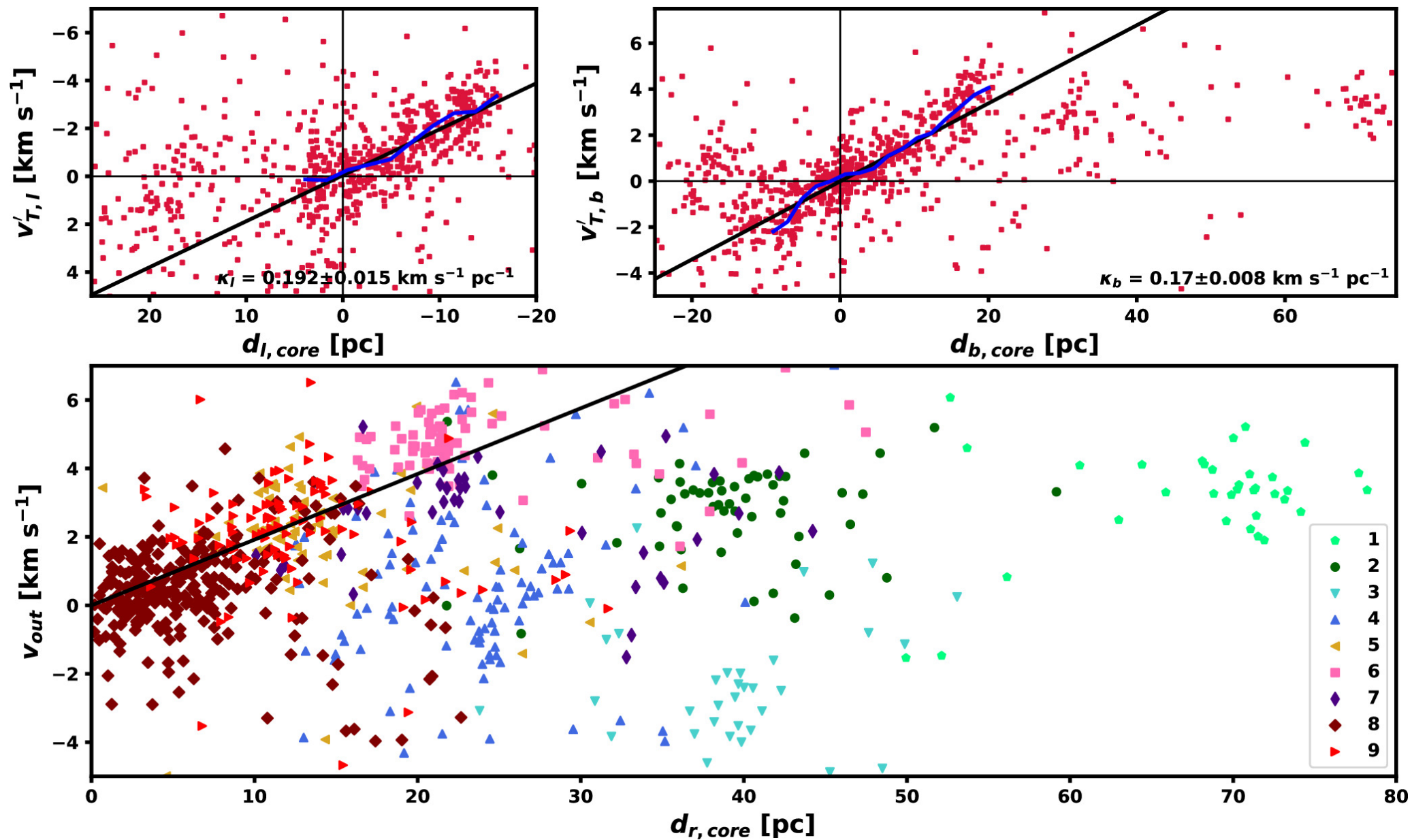
Figure 10. from Ronan Kerr et al 2025 Astrophys. J. 985 doi:10.3847/1538-4357/adc0a7 https://dx.doi.org/10.3847/1538-4357/adc0a7 © 2025. The Author(s). Published by the American Astronomical Society.
