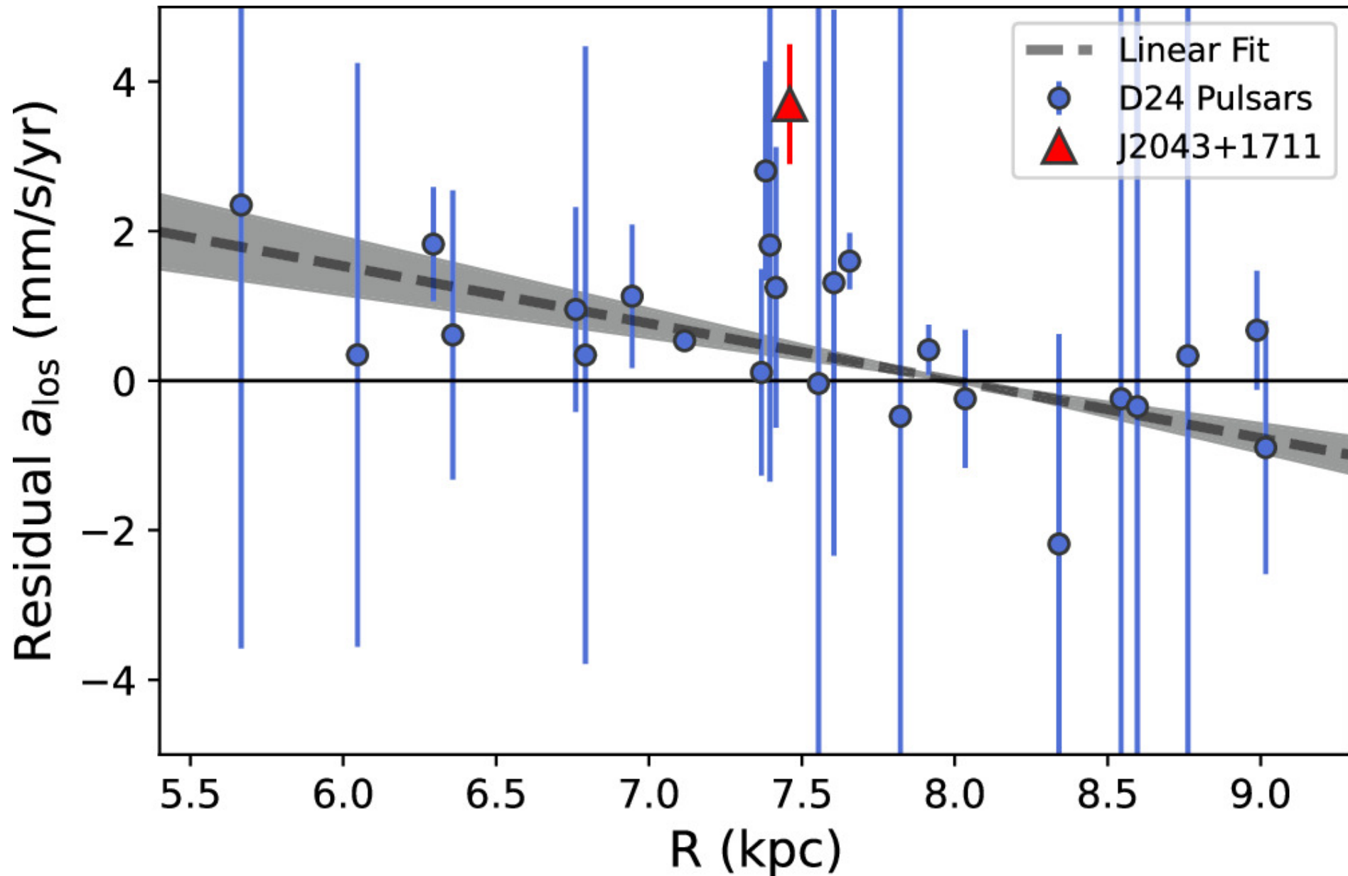
Figure 6. from Thomas Donlon et al 2025 Astrophys. J. 983 doi:10.3847/1538-4357/adbf90 https://dx.doi.org/10.3847/1538-4357/adbf90 © 2025. The Author(s). Published by the American Astronomical Society.
