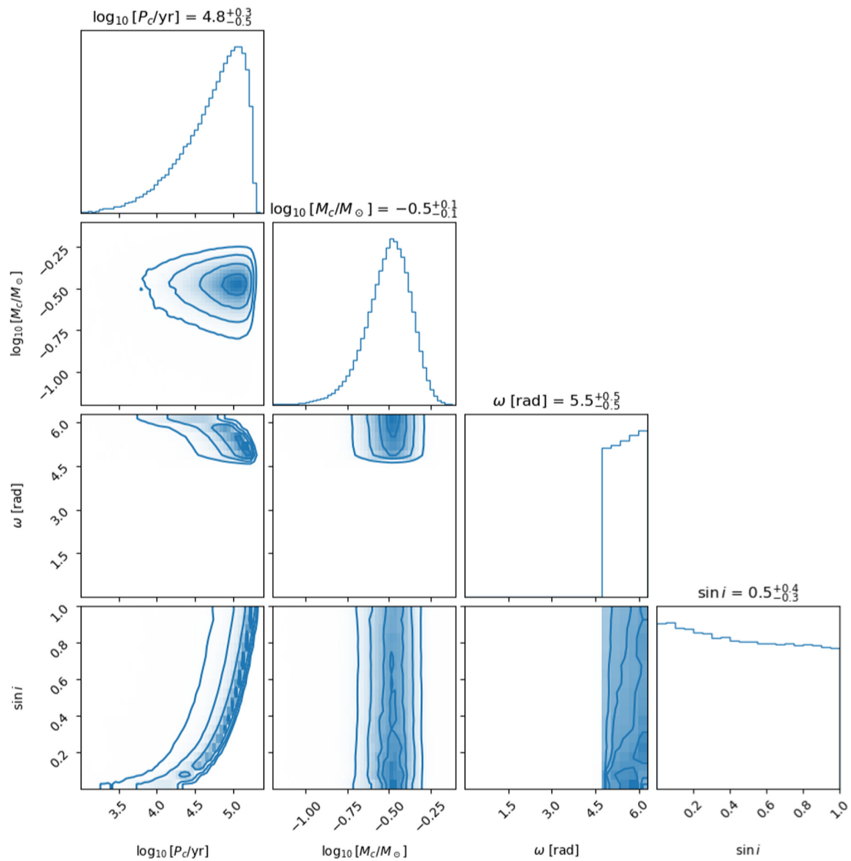
Figure 4. from Thomas Donlon et al 2025 Astrophys. J. 983 doi:10.3847/1538-4357/adbf90 https://dx.doi.org/10.3847/1538-4357/adbf90 © 2025. The Author(s). Published by the American Astronomical Society.
