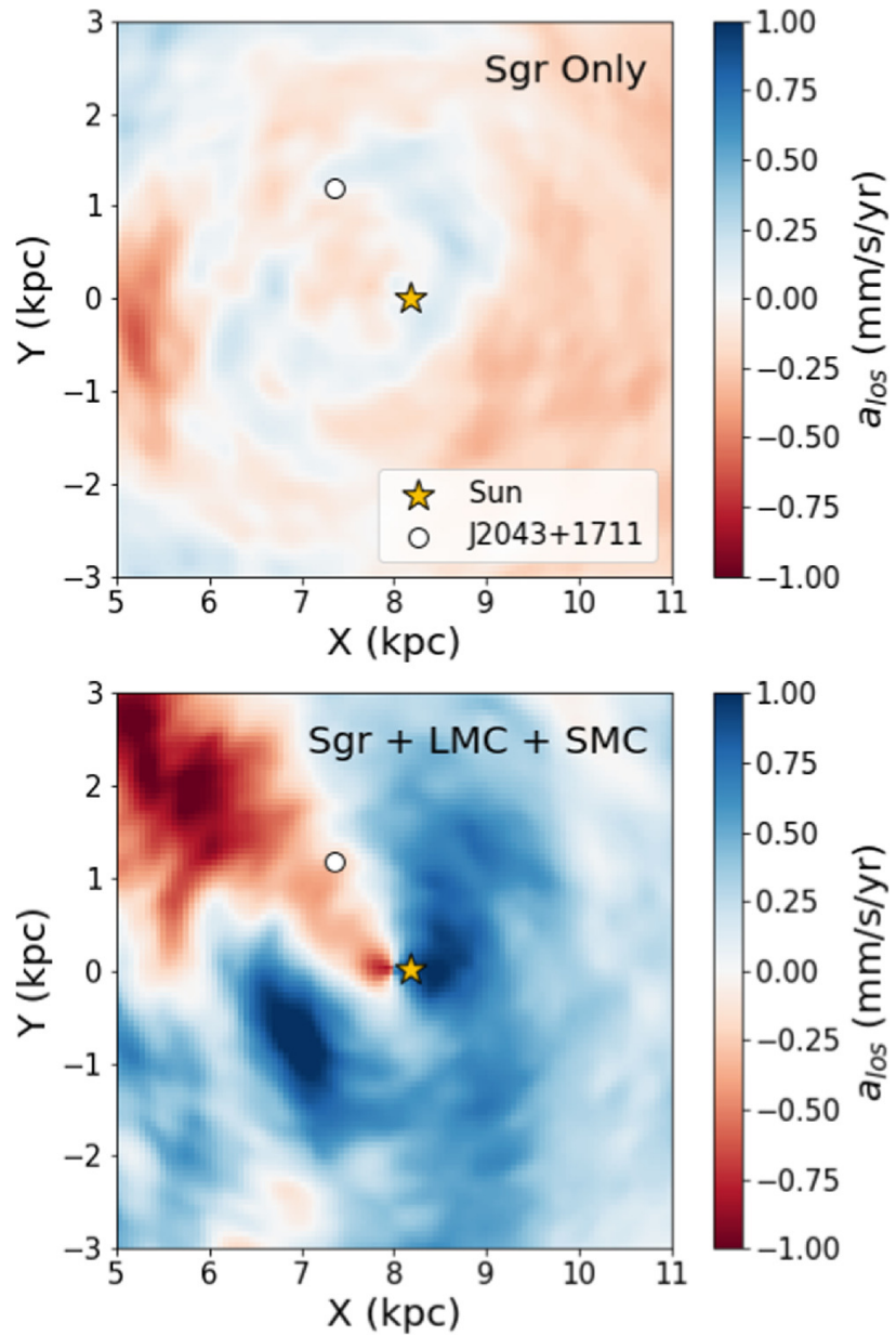
Figure 1. from Thomas Donlon et al 2025 Astrophys. J. 983 doi:10.3847/1538-4357/adbf90 https://dx.doi.org/10.3847/1538-4357/adbf90 © 2025. The Author(s). Published by the American Astronomical Society.
