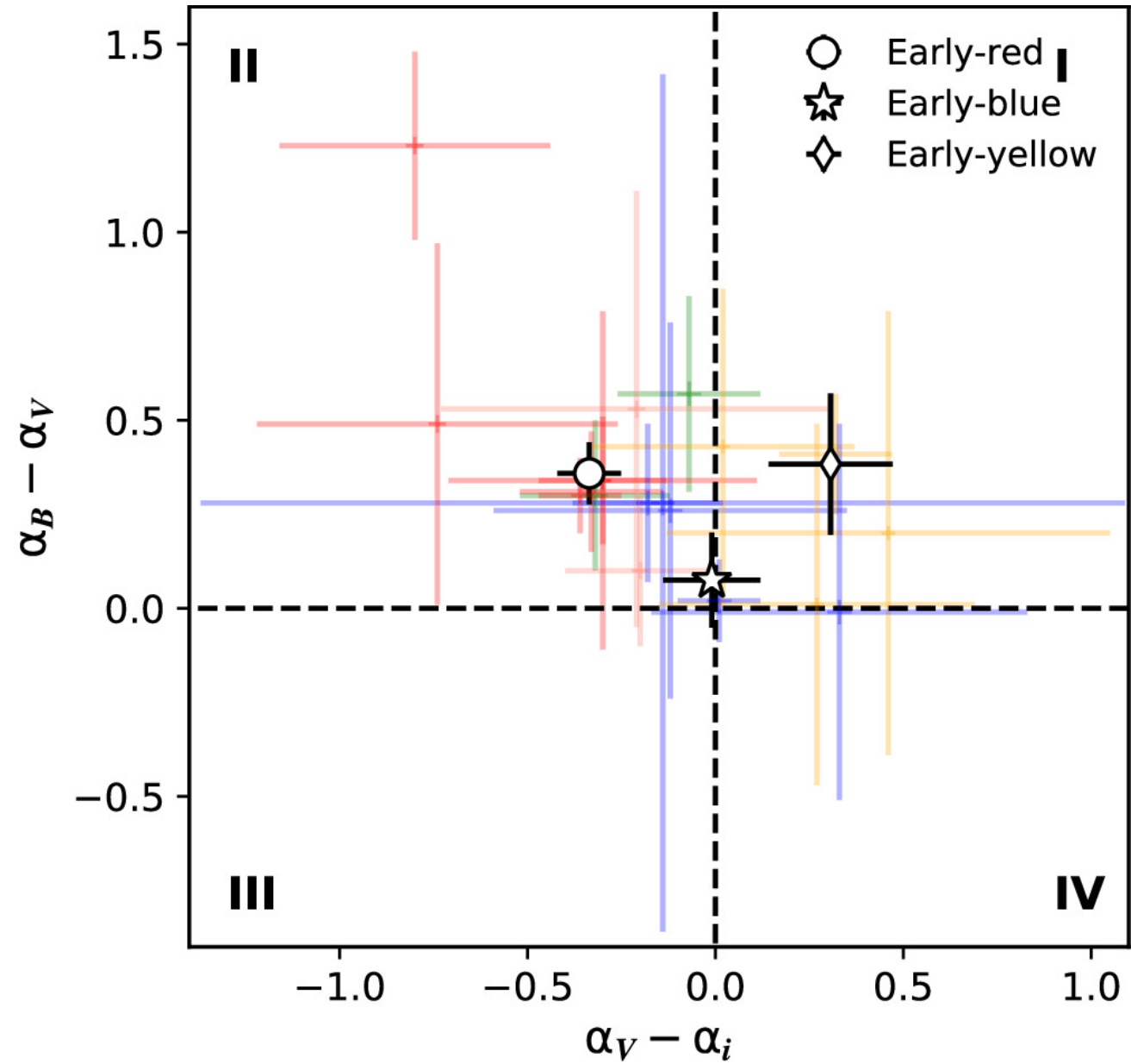
Figure 8. from Yuan Qi Ni et al 2025 Astrophys. J. 983 doi:10.3847/1538-4357/adbbb7 https://dx.doi.org/10.3847/1538-4357/adbbb7 © 2025. The Author(s). Published by the American Astronomical Society.
