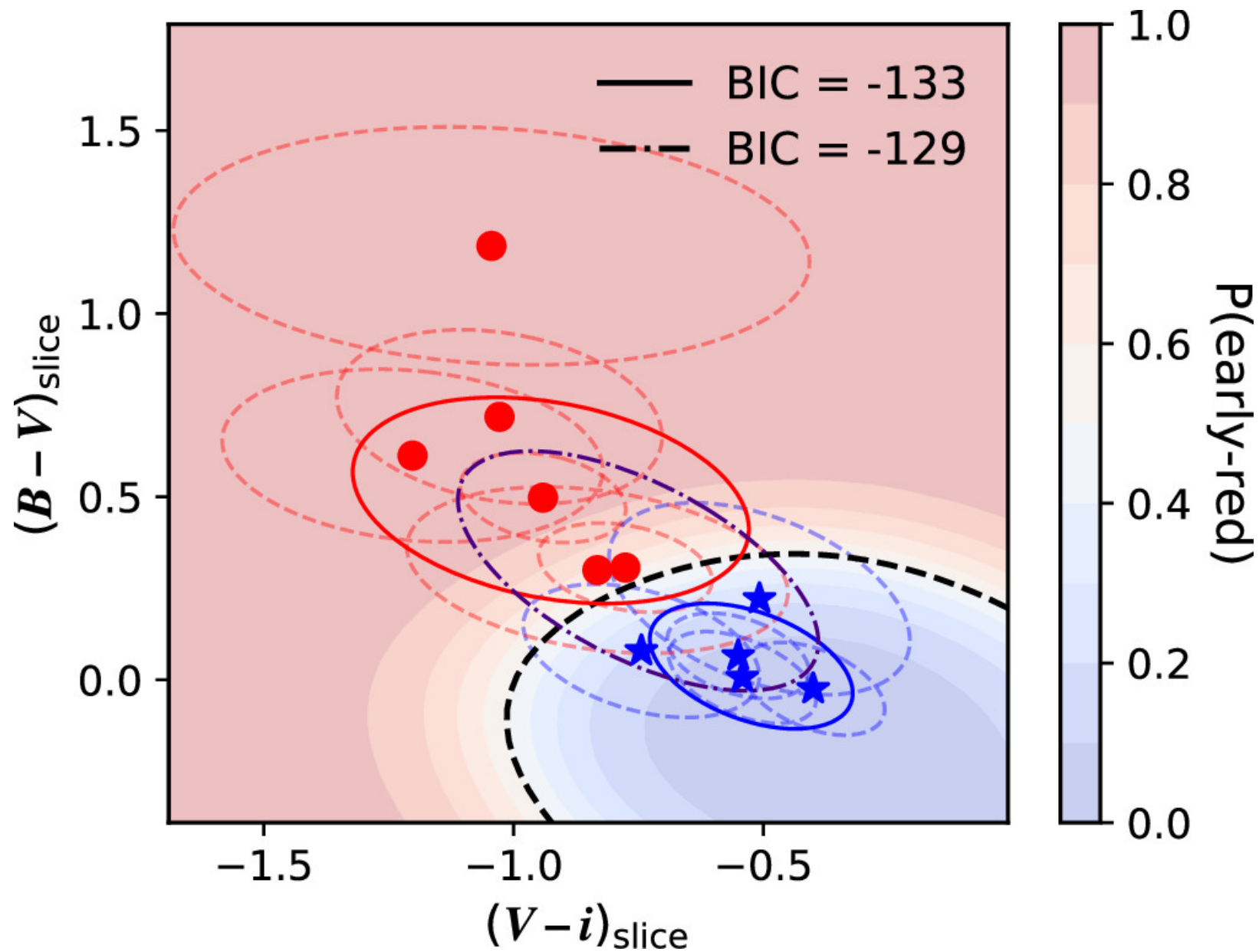
Figure 7. from Yuan Qi Ni et al 2025 Astrophys. J. 983 doi:10.3847/1538-4357/adbbb7 https://dx.doi.org/10.3847/1538-4357/adbbb7 © 2025. The Author(s). Published by the American Astronomical Society.
