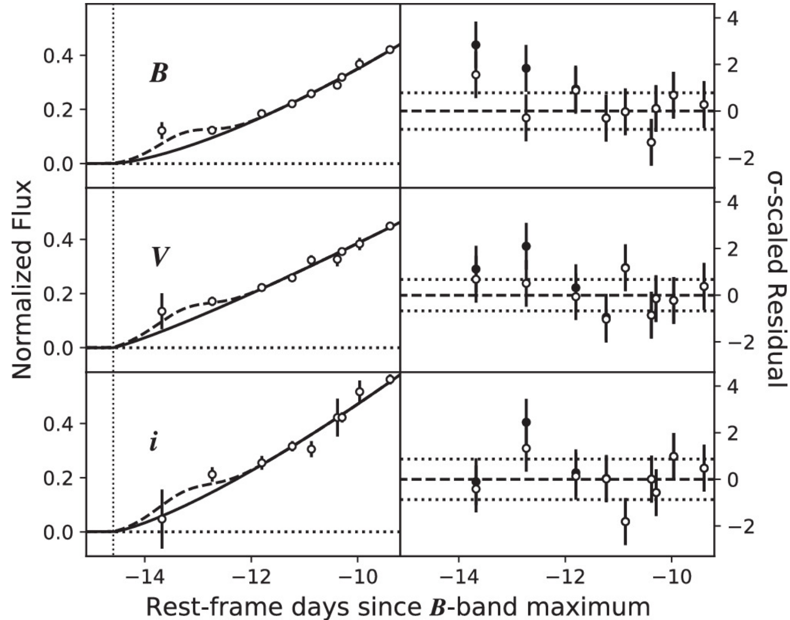
Figure 4. from Yuan Qi Ni et al 2025 Astrophys. J. 983 doi:10.3847/1538-4357/adbbb7 https://dx.doi.org/10.3847/1538-4357/adbbb7 © 2025. The Author(s). Published by the American Astronomical Society.
