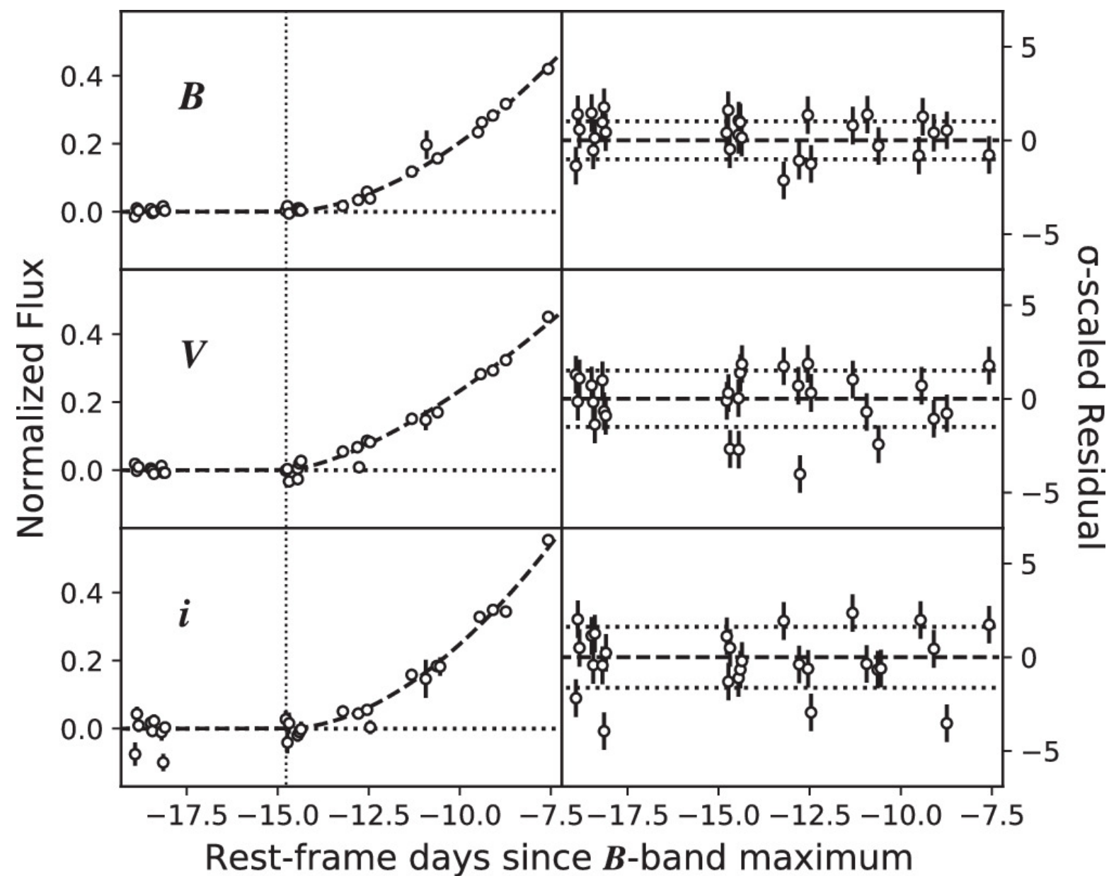
Figure 3. from Yuan Qi Ni et al 2025 Astrophys. J. 983 doi:10.3847/1538-4357/adbbb7 https://dx.doi.org/10.3847/1538-4357/adbbb7 © 2025. The Author(s). Published by the American Astronomical Society.
