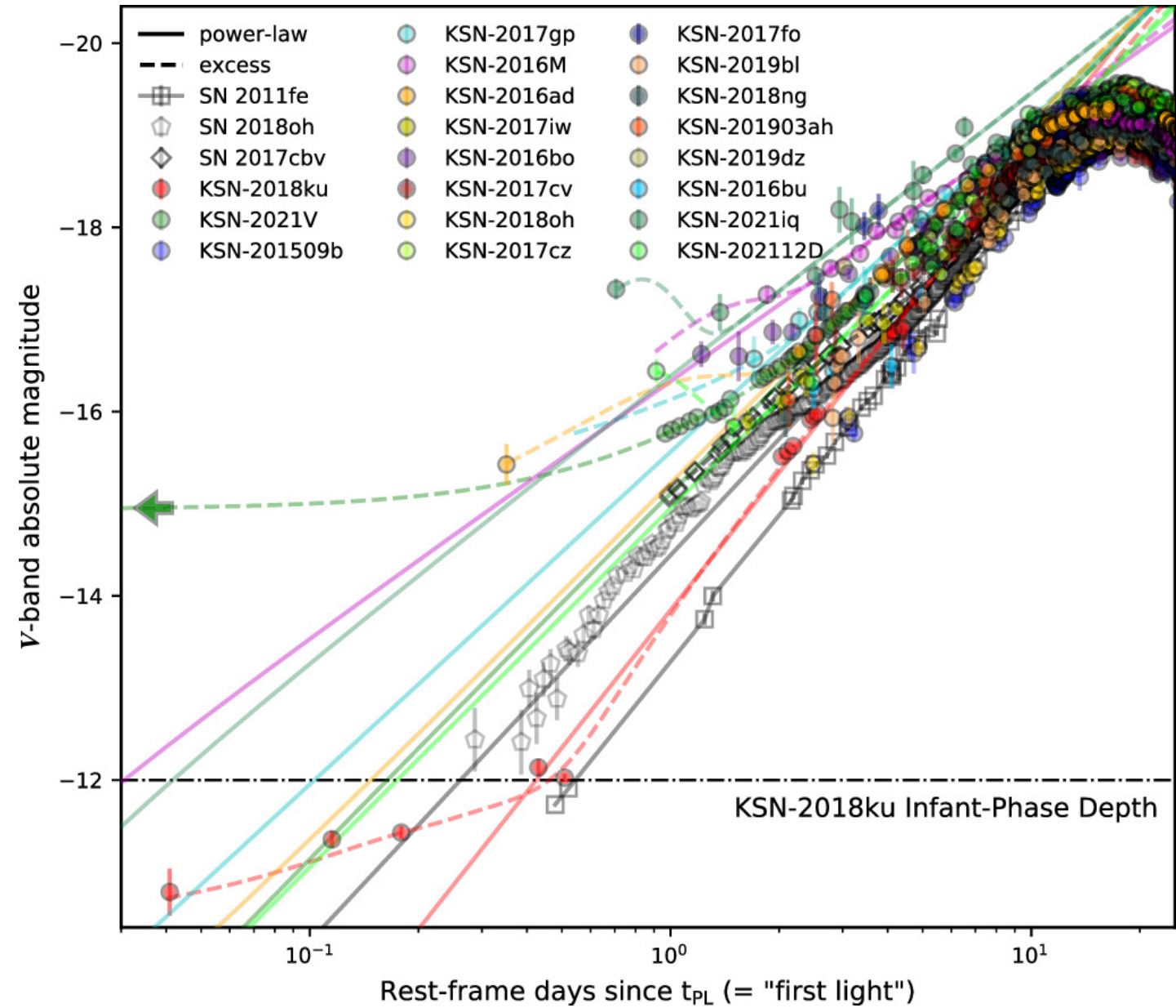
Figure 2. from Yuan Qi Ni et al 2025 Astrophys. J. 983 doi:10.3847/1538-4357/adbbb7 https://dx.doi.org/10.3847/1538-4357/adbbb7 © 2025. The Author(s). Published by the American Astronomical Society.
