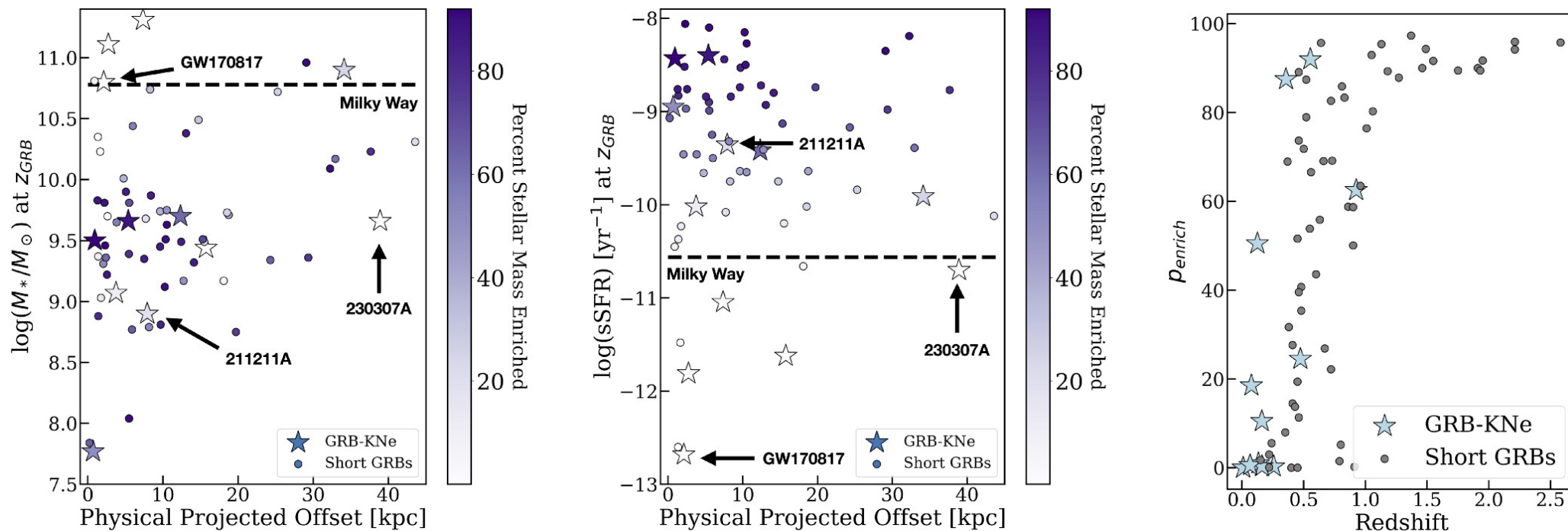
Figure 7. from Anya E. Nugent et al 2025 Astrophys. J. 982 doi:10.3847/1538-4357/adbb6a https://dx.doi.org/10.3847/1538-4357/adbb6a © 2025. The Author(s). Published by the American Astronomical Society.
