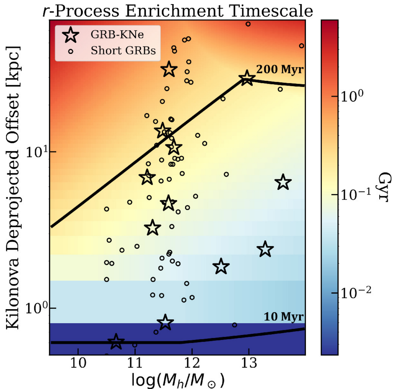
Figure 4. from Anya E. Nugent et al 2025 Astrophys. J. 982 doi:10.3847/1538-4357/adbb6a https://dx.doi.org/10.3847/1538-4357/adbb6a © 2025. The Author(s). Published by the American Astronomical Society.
