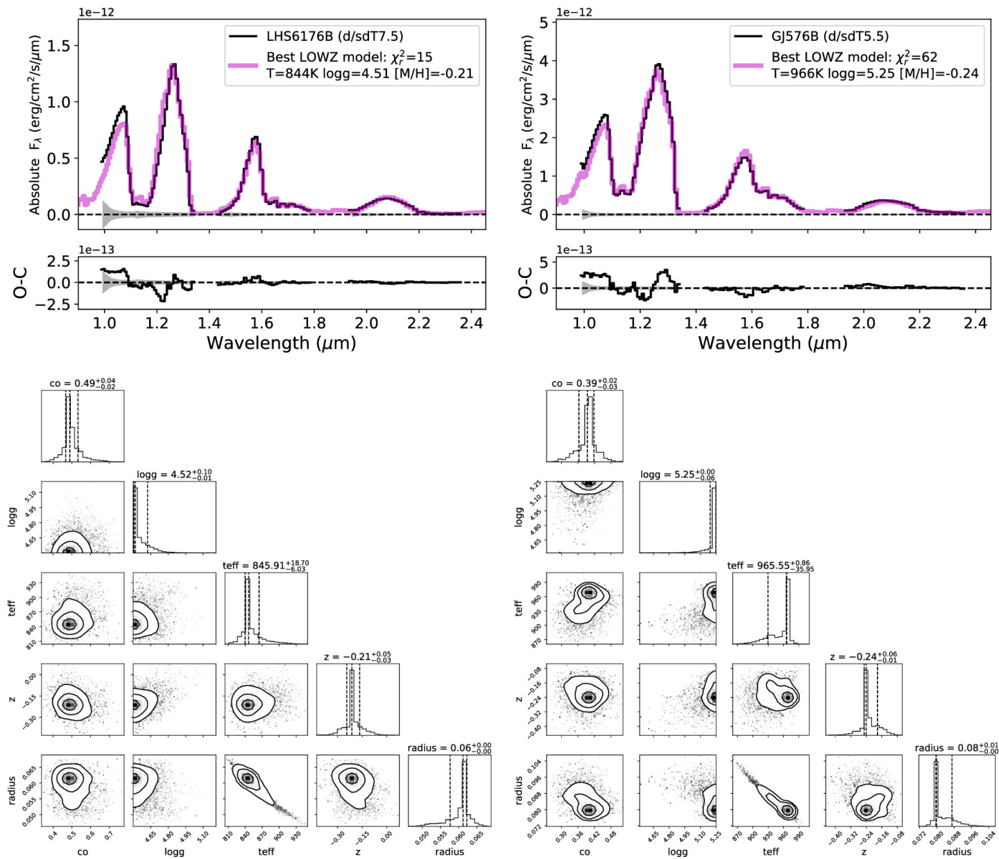
Figure 6. from Adam J. Burgasser et al 2025 Astrophys. J. 982 doi:10.3847/1538-4357/adb39f https://dx.doi.org/10.3847/1538-4357/adb39f © 2025. The Author(s). Published by the American Astronomical Society.
