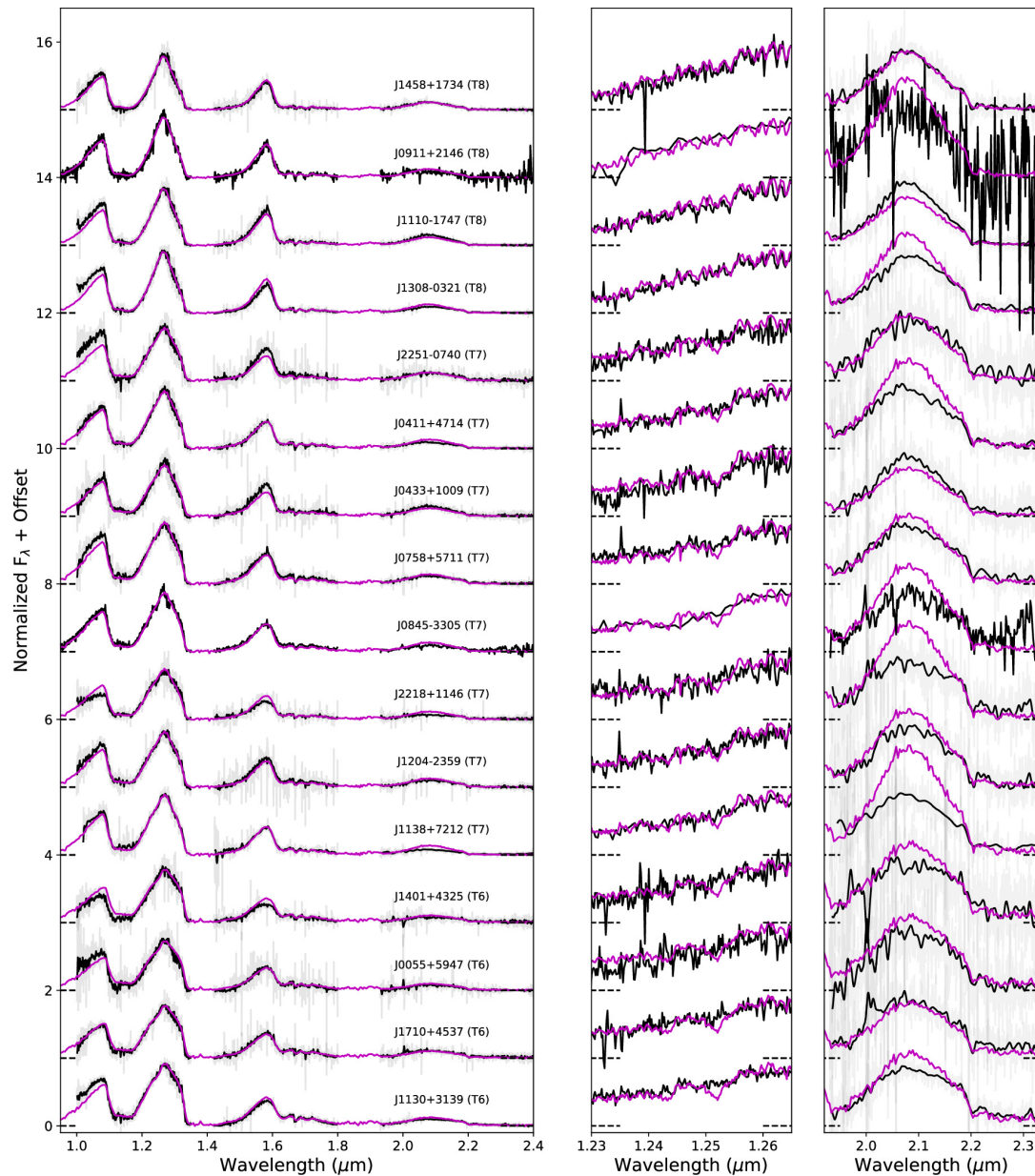
Figure 4. from Adam J. Burgasser et al 2025 Astrophys. J. 982 doi:10.3847/1538-4357/adb39f https://dx.doi.org/10.3847/1538-4357/adb39f © 2025. The Author(s). Published by the American Astronomical Society.
