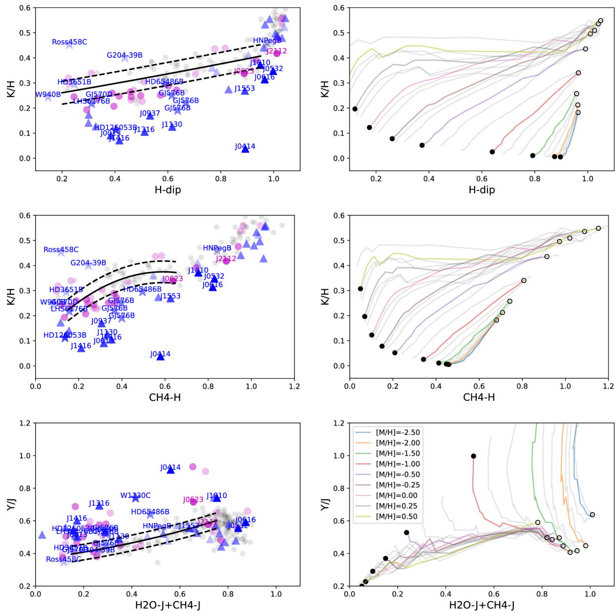
Figure 16. from Adam J. Burgasser et al 2025 Astrophys. J. 982 doi:10.3847/1538-4357/adb39f https://dx.doi.org/10.3847/1538-4357/adb39f © 2025. The Author(s). Published by the American Astronomical Society.
