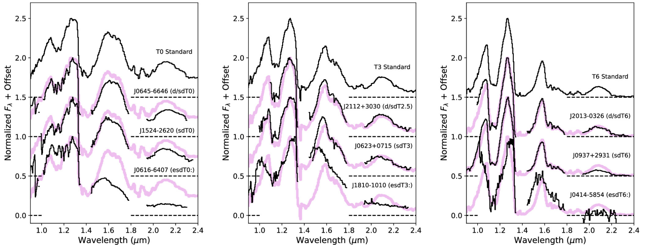
Figure 14. from Adam J. Burgasser et al 2025 Astrophys. J. 982 doi:10.3847/1538-4357/adb39f https://dx.doi.org/10.3847/1538-4357/adb39f © 2025. The Author(s). Published by the American Astronomical Society.
