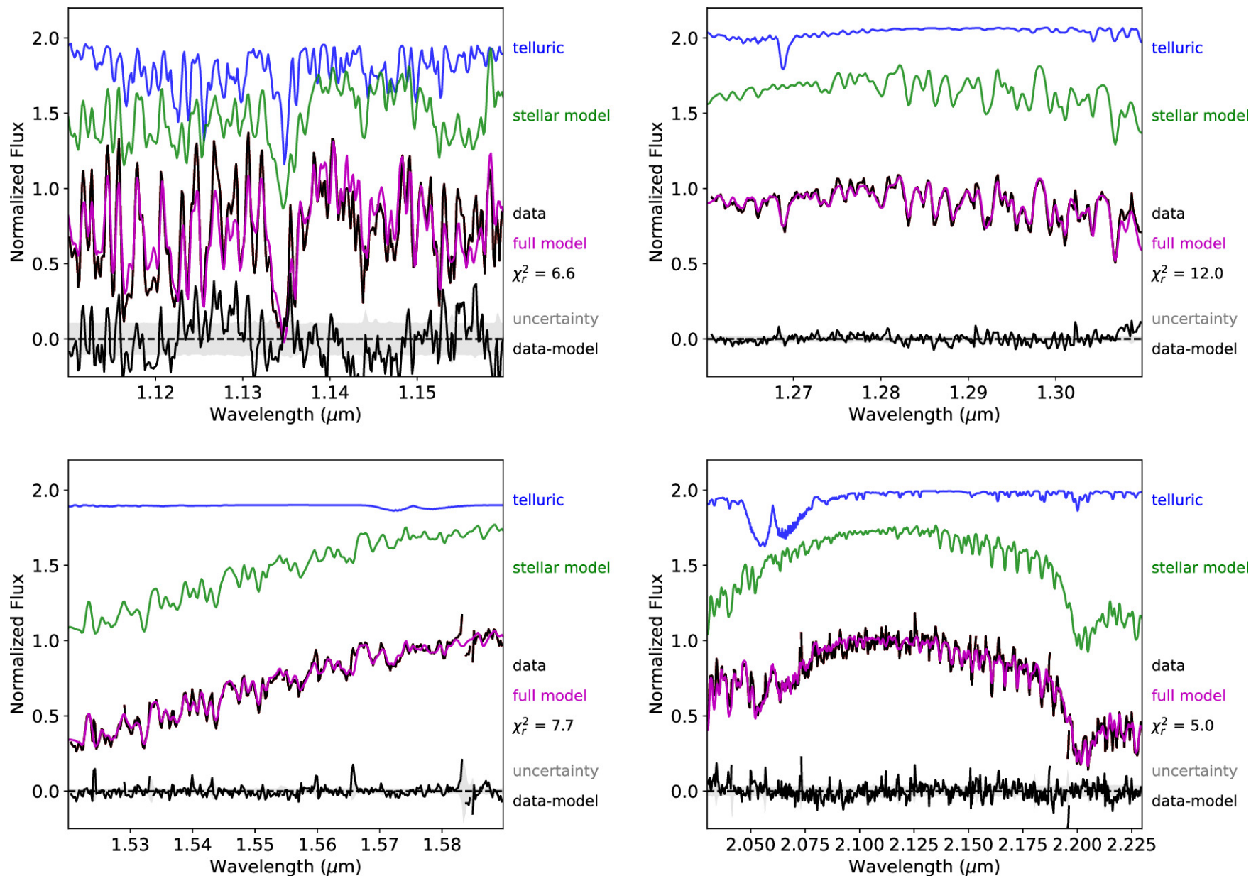
Figure 10. from Adam J. Burgasser et al 2025 Astrophys. J. 982 doi:10.3847/1538-4357/adb39f https://dx.doi.org/10.3847/1538-4357/adb39f © 2025. The Author(s). Published by the American Astronomical Society.
