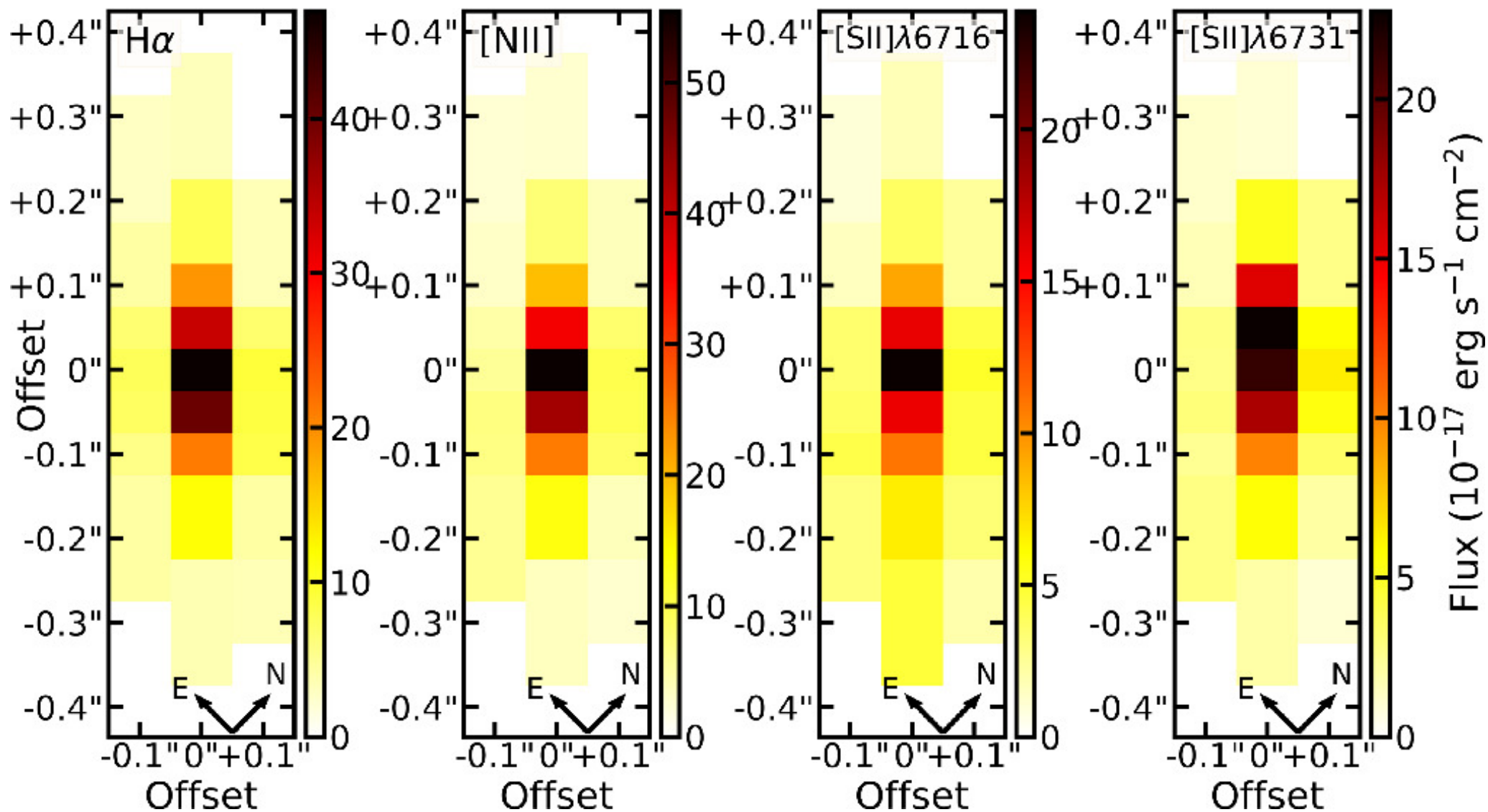
Figure 8. from Julie Hlavacek-Larrondo et al 2025 Astrophys. J. 980 doi:10.3847/1538-4357/ada7ed https://dx.doi.org/10.3847/1538-4357/ada7ed © 2025. The Author(s). Published by the American Astronomical Society.
