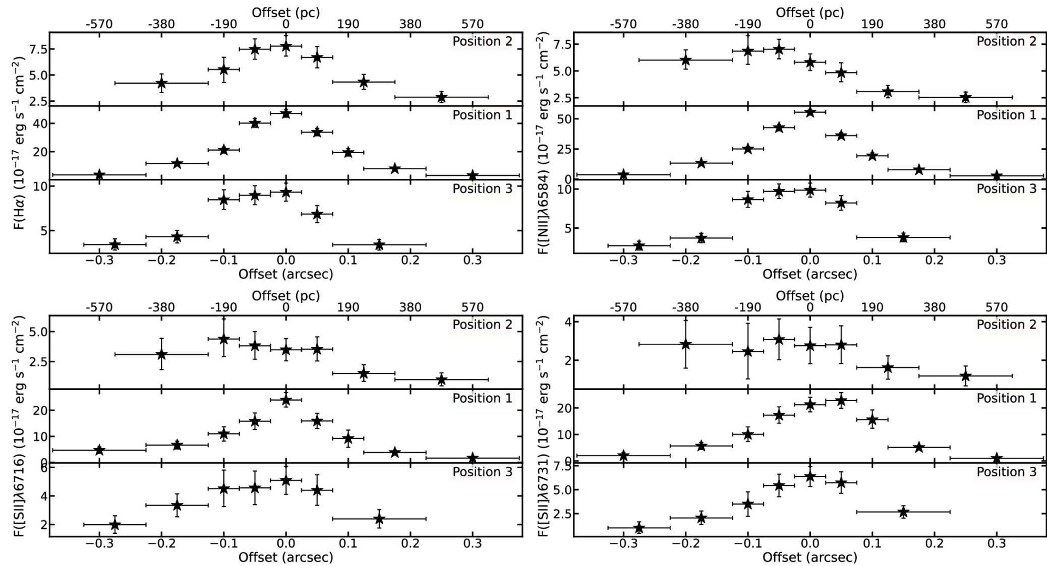
Figure 7. from Julie Hlavacek-Larrondo et al 2025 Astrophys. J. 980 doi:10.3847/1538-4357/ada7ed https://dx.doi.org/10.3847/1538-4357/ada7ed © 2025. The Author(s). Published by the American Astronomical Society.
